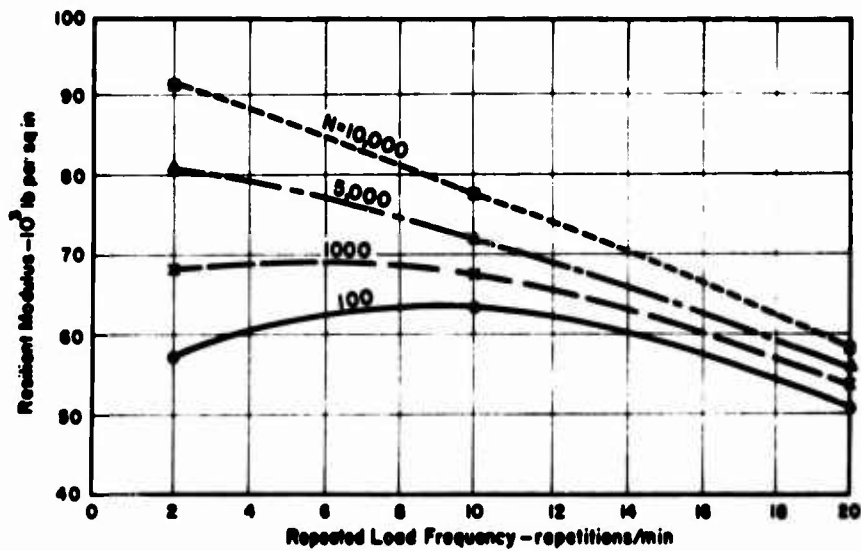
(b) Repeated Stress Level = 60 percent
