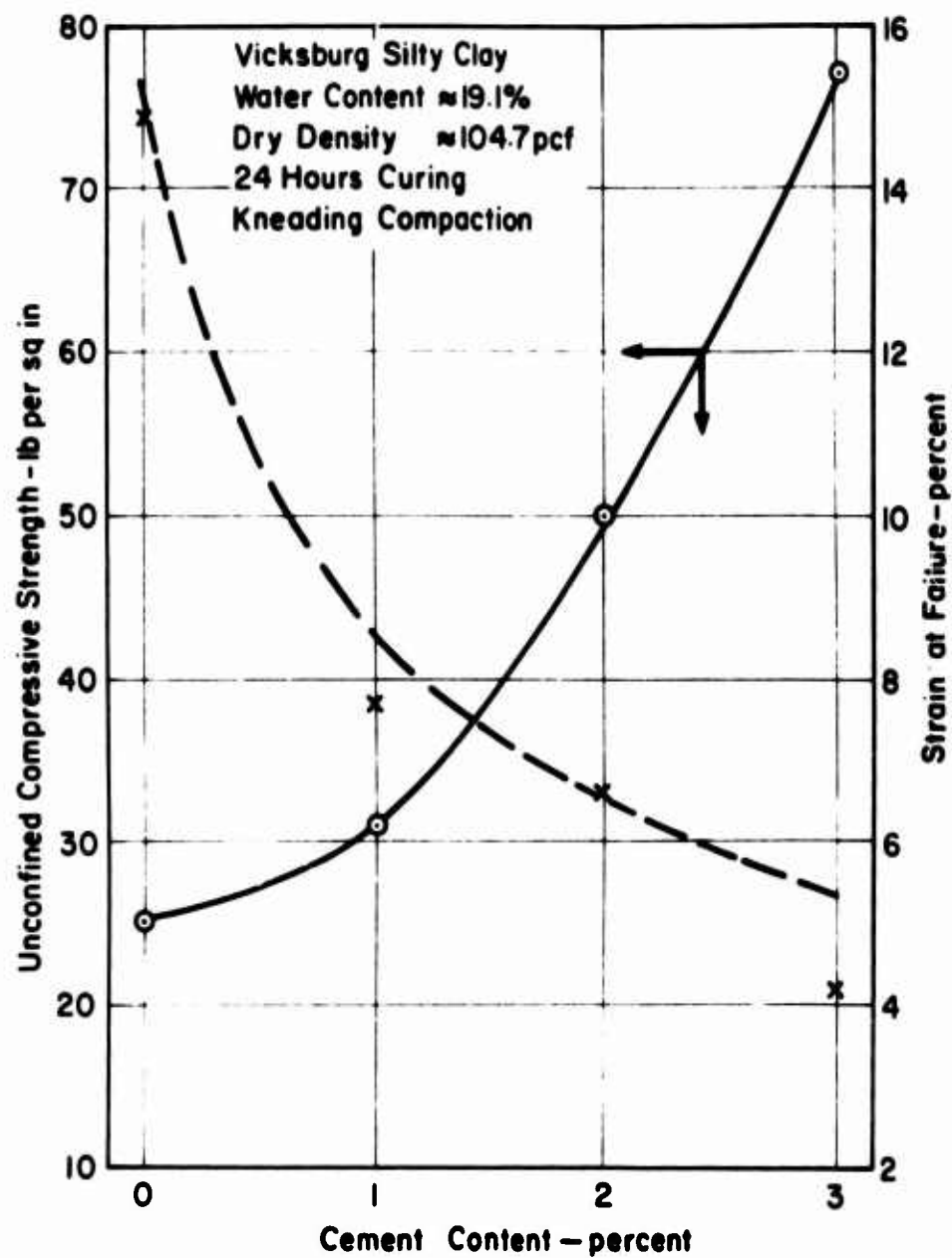
FIG.57— UNCONFINED COMPRESSIVE STRENGTH AS A FUNCTION OF CEMENT CONTENT.
