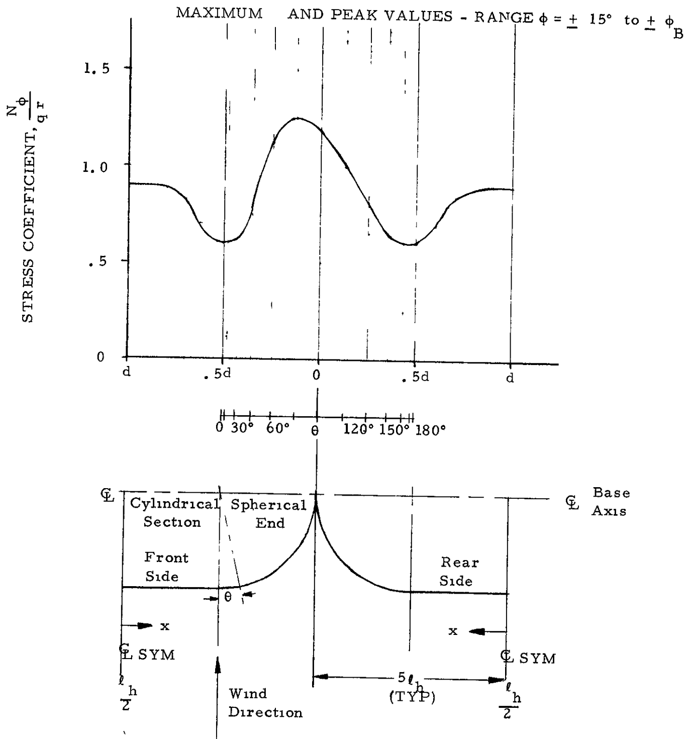
FIGURE 67. - TYPICAL ANNULAR - LONGITUDINAL STRESS COEFFICIENT DISTRIBUTION MODEL NO. 8 - ALL TESTS.
