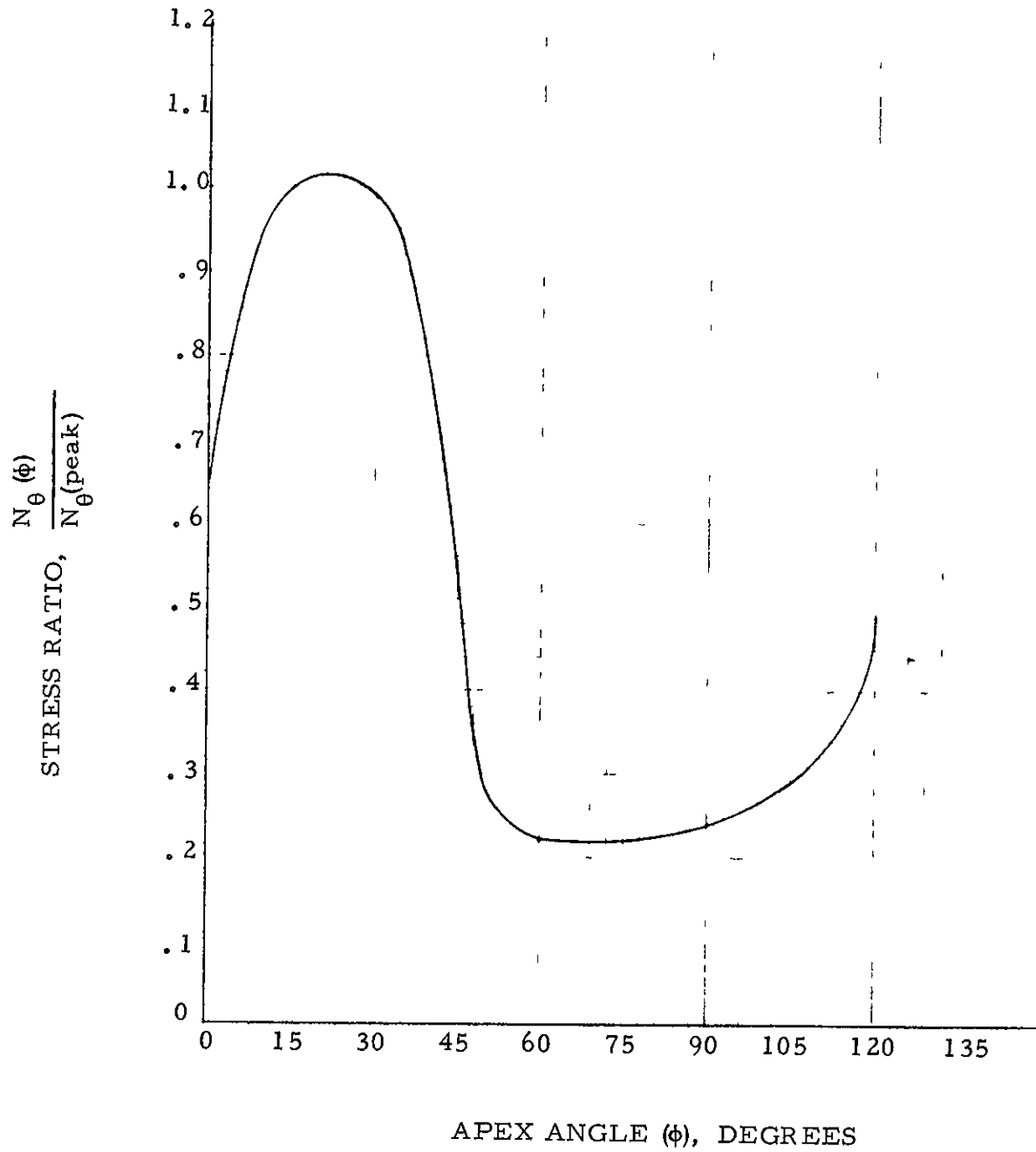
FIGURE 58. - STRESS RATIO, \frac{N_{\theta}(\phi)}{N_{\theta}(\text{peak})} VS. APEX ANGLE, \phi
