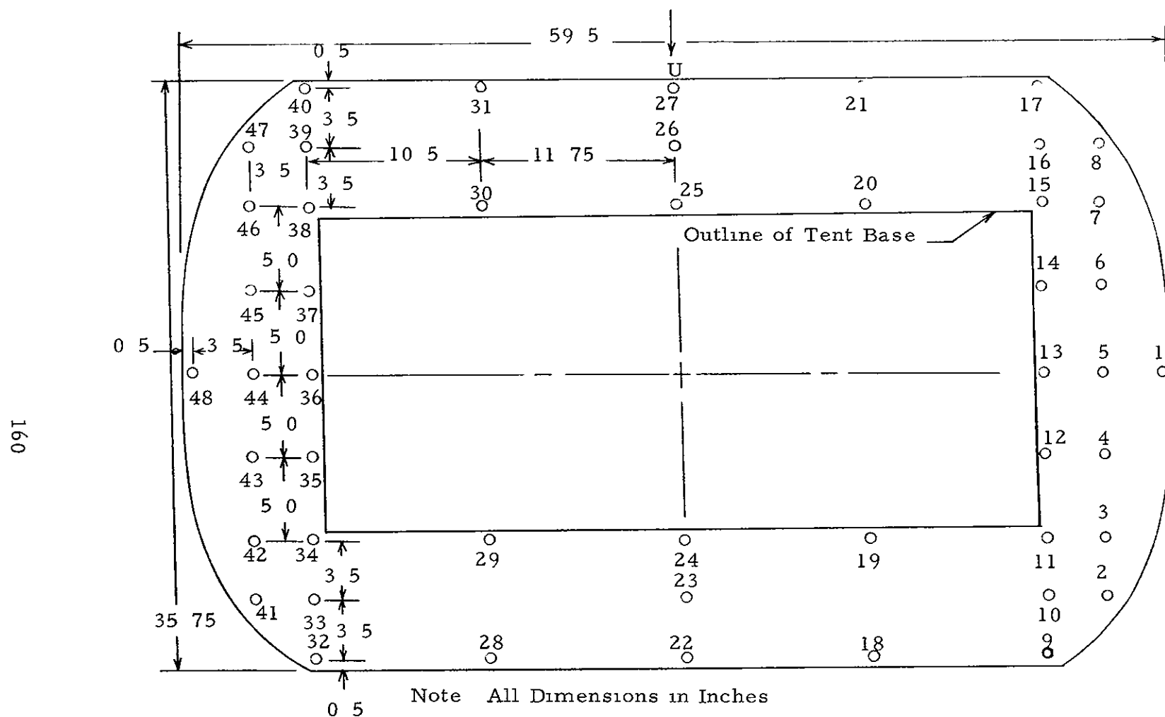
FIGURE 85 - PICKUP LOCATIONS FOR PRESSURE DISTRIBUTION MEASUREMENT ON MODEL BASE FOR MODEL NO 19
