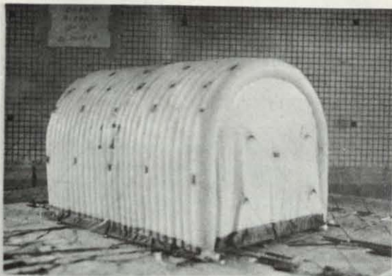
Model No. 17 3/4 Cylinder Cell Width/Enclosure Dia. = 0.082
