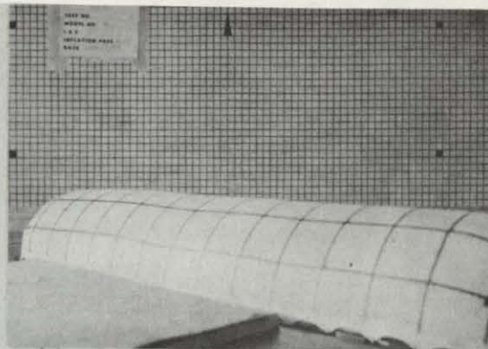
Model No. 6 1/2 Cylinder
