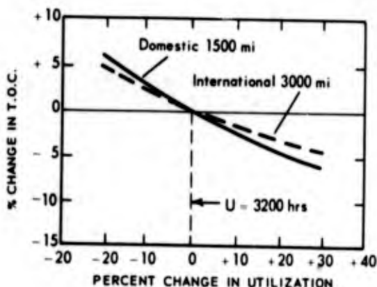
Fig. 12—Utilization Sensitivity
