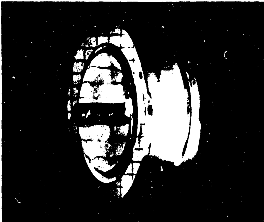
Figure B-14. Extrusion of the unsupported low pressure face of a 0.735-inch-thick, 0.490 t/D; ratio window subjected to 18,600 psi pressure.
