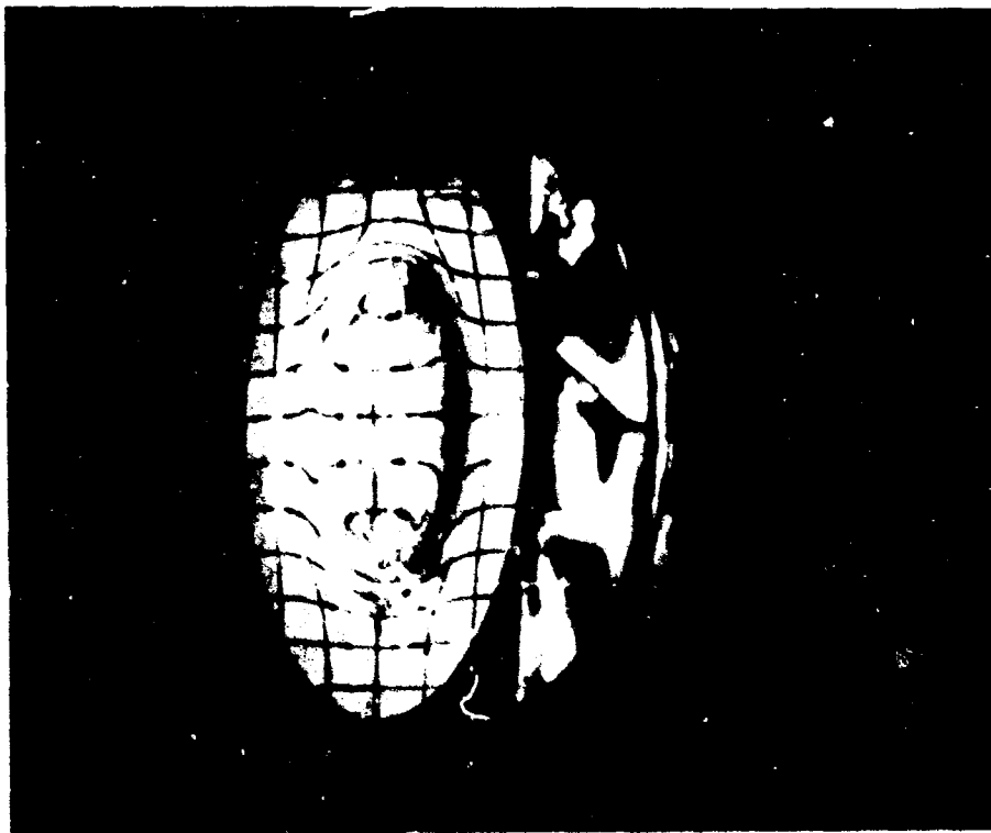
Figure B-13. Plastic flow cratering on the high-pressure side of a 0.735-inch-thick, 0.490 t/D; ratio window subjected to 18,600 psi pressure.
