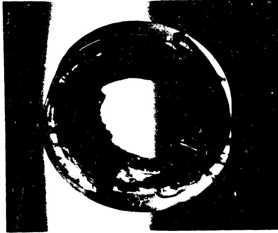
Figure 8-16. Shear-type failure in a 1.432-inch-thick, 0.500 t/D_i ratio window which failed at 15,300 psi.
