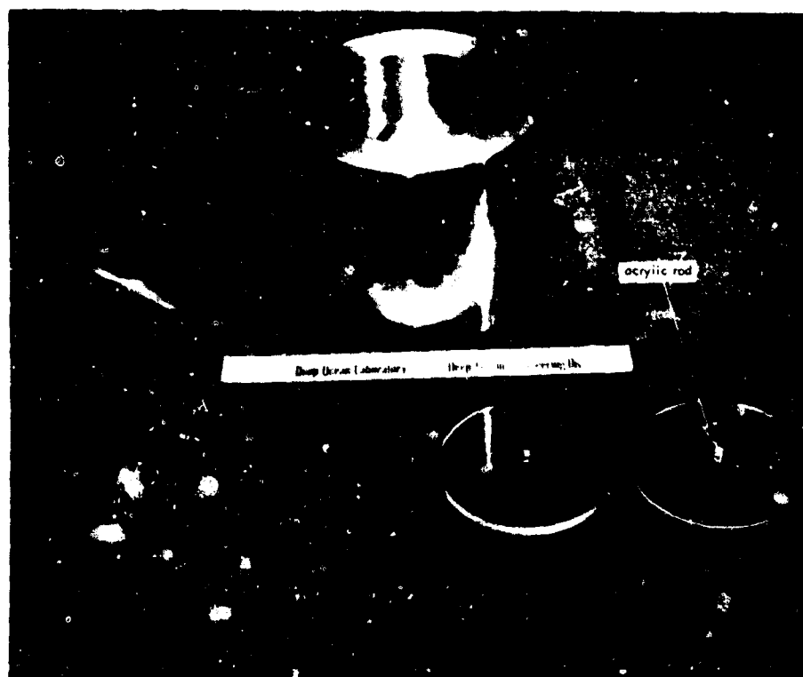
Figure 3. Flat acrylic windows and 3.53-inch ( D_i ) flange used to determine the relationship between the window's critical pressure and t/D_i ratio.
