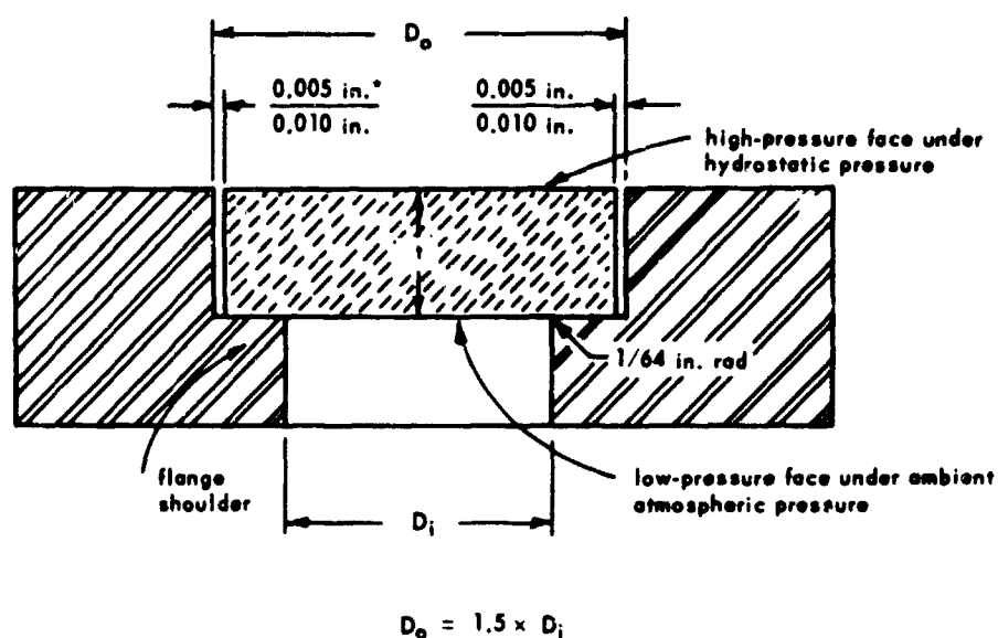
Figure 1. DOL type III flange configuration for short-term testing of flat acrylic windows.
