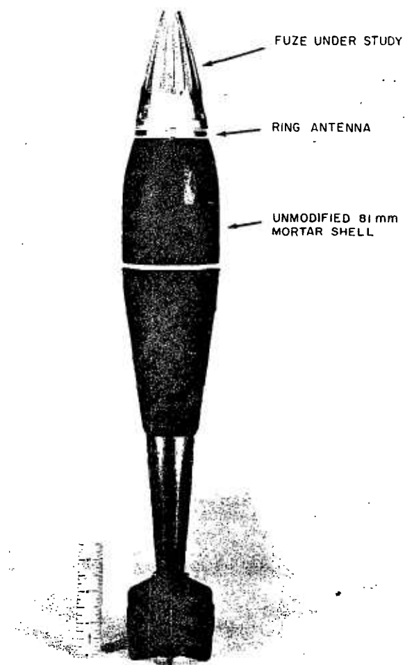
674-66 Fig.1 Ring Antenna Mounted on 81-mm Mortar Shell.
