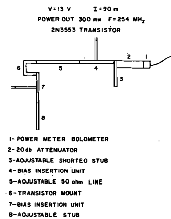
Figure 5. Coaxial oscillator
