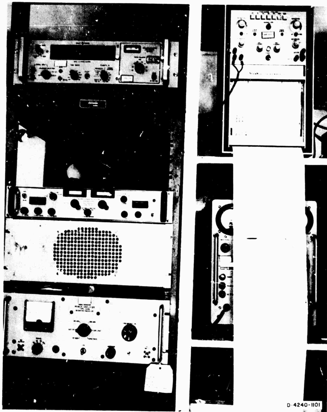
FIG. 3 RECEIVING EQUIPMENT IN TEST VAN (Left rack, top to bottom; Hewlett-Pockord 5245 counter, Astra Cammunications Lobarotary SCR202 VHF receiver, Boanton 230A power amplifier; right rack, top to bottom: Brush Mark 2500 recorder, Hewlett-Pockard 608D VHF signal generatar.)
