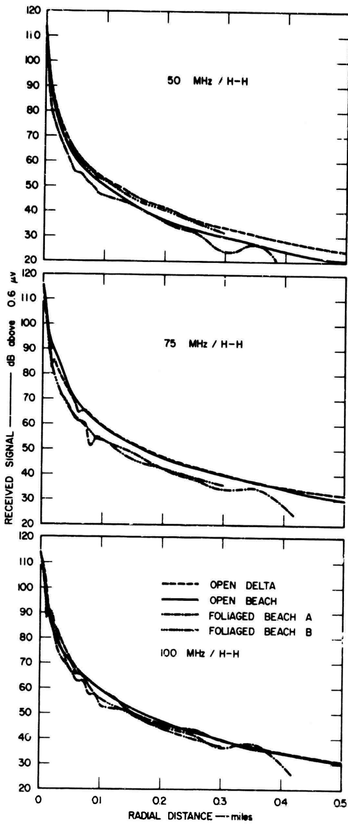
FIG. 24 TERRAIN COMPARISONS FOR HORIZONTAL POLARIZATION
