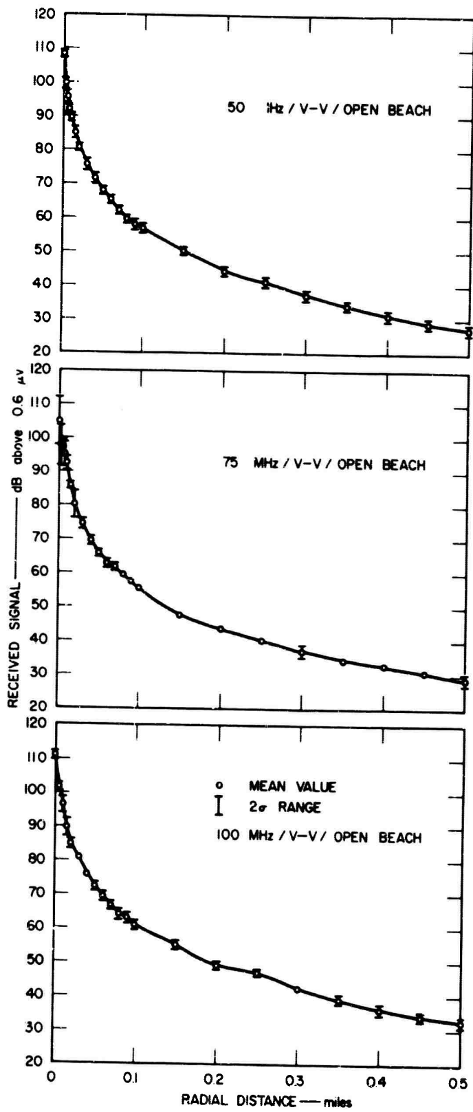
FIG. 11 BASIC CURVES FOR VERTICAL POLARIZATION, OPEN BEACH
