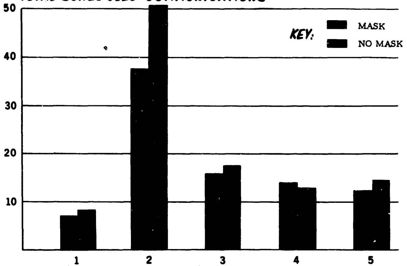
Figure 9. Average number of total scheduled signals per subtask.
