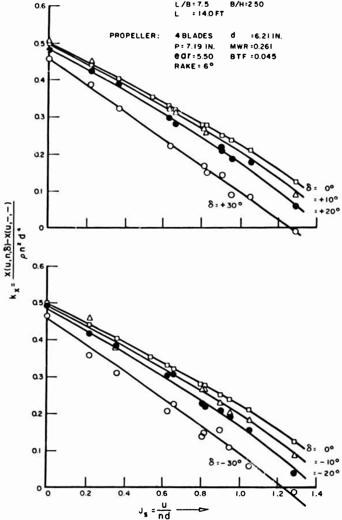
FIGURE 2. VARIATION OF LONGITUDINAL FORCE COEFFICIENT k_x , WITH RUDDER ANGLE AND PROPELLER ADVANCE-RATIO IN BEHIND-SHIP CONDITION
