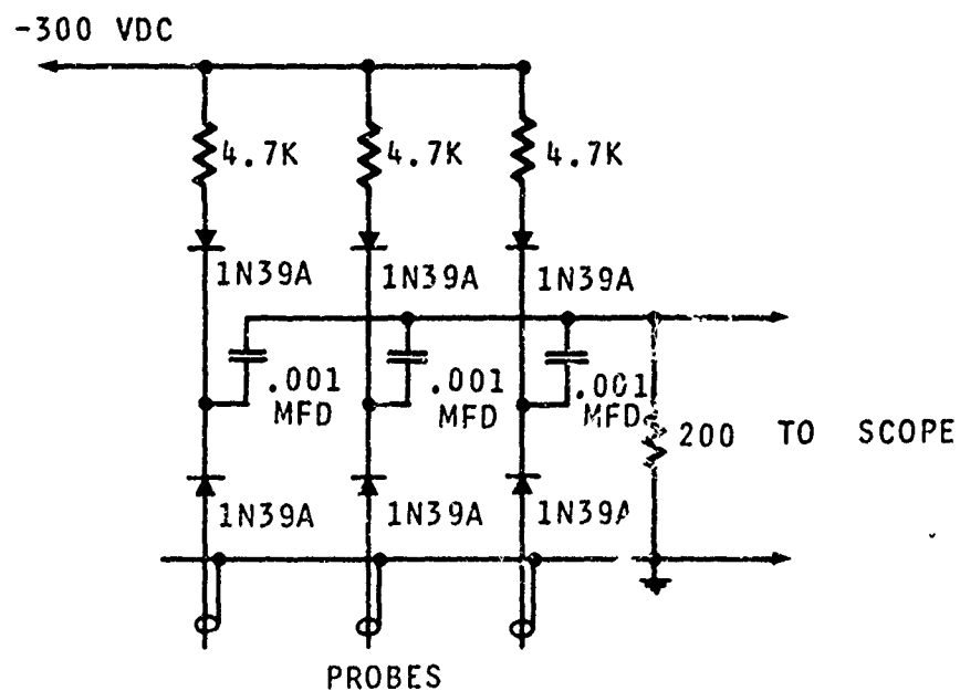
B. IONIZATION PROBE CIRCUIT AS MODIFIED TO DETECT REFLECTED WAVES
