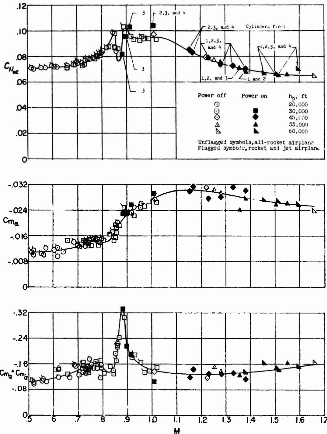
Fig. 54 Variation of static and dynamic longitudinal stability derivatives of the D-558-II airplane with Mach number (from Reference 43)
