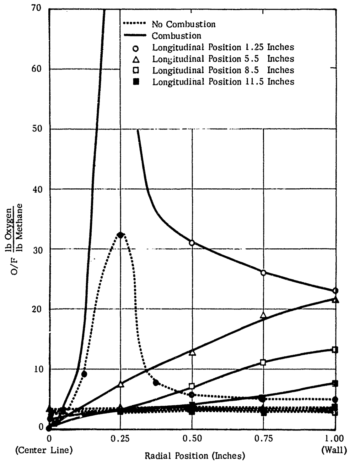
FIGURE 12 13-INCH MOTOR--MIXTURE RATIO GRADIENTS (WITH OR WITHOUT COMBUSTION)
