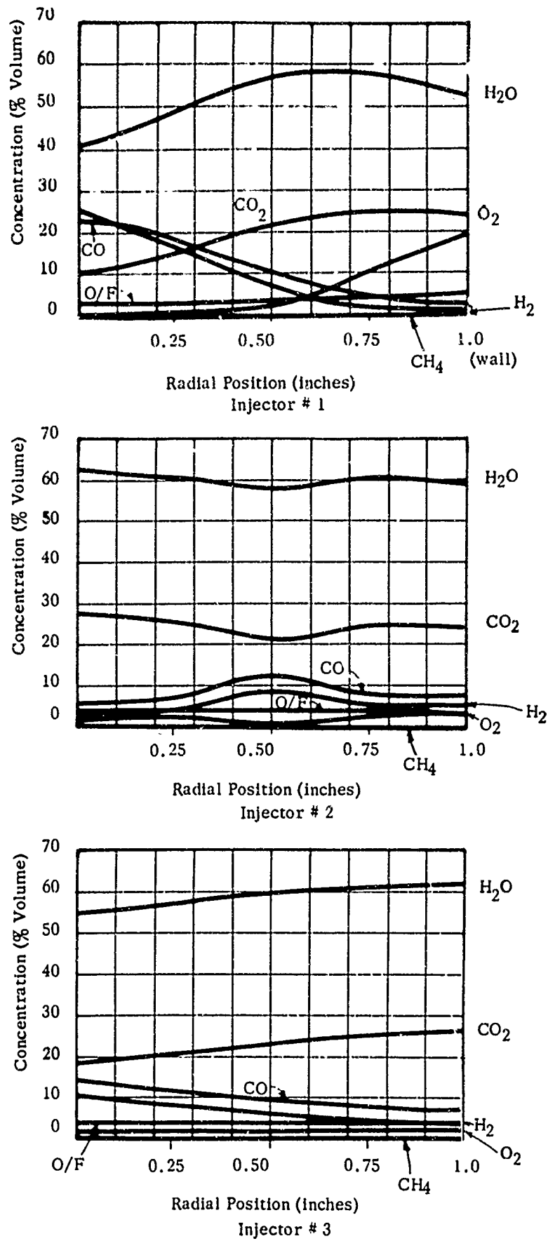
FIGURE 10 MOTOR 16 INCHES -- Radial Concentration Gradients at Longitudinal Position 14.5 Inches
