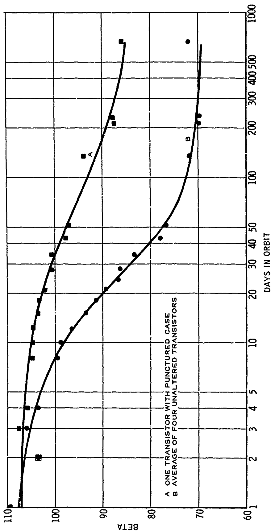
Fig. 6 Beta versus Time for Fairchild 2N1711 NPN Planar Transistors Flown on 1963-38C Satellite
