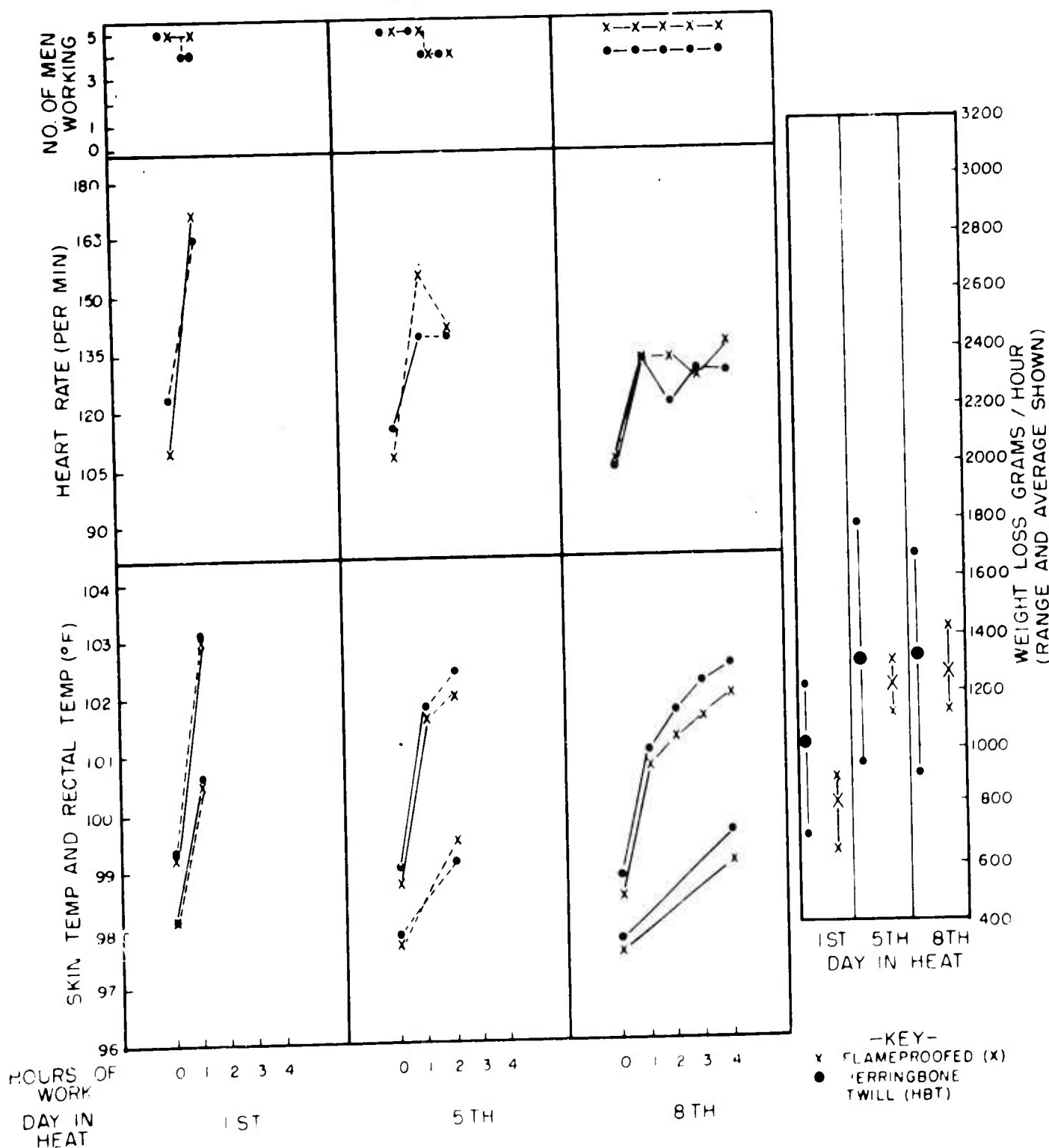
CHART I AVERAGE PHYSIOLOGIC RESPONSE OF WORKING MEN WEARING FLAMEPROOFED (X) TWILL AND HERRINGBONE TWILL D.B. 120° F - W.B. 88° F
