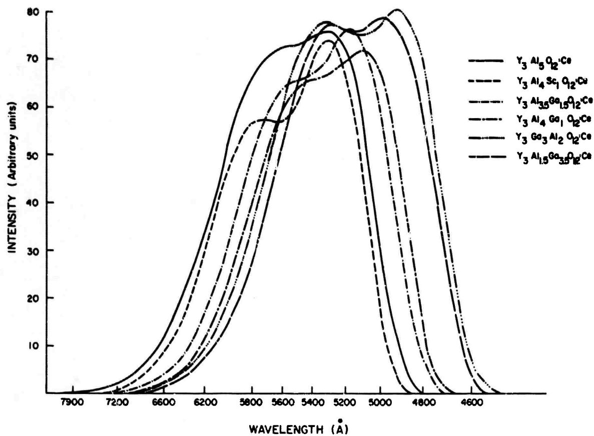
FIG. 4 Comparison of the low temperature fluorescence of cerium doped \text{Y}_3\text{Al}_5\text{O}_{12} with the fluorescences observed in cerium doped garnet crystals where the \text{Al}^{3+} ions have been replaced by \text{Ga}^{3+} or \text{Sc}^{3+} ions. These profiles were measured at 77°K.
