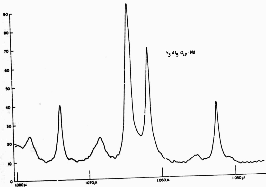
FIG. 1 The spectrum of the {}^4F_{3/2} \rightarrow {}^4I_{11/2} fluorescent transitions of the \text{Nd}^{3+} ion in \text{Y}_3\text{Al}_5\text{O}_{12} measured at room temperature.
