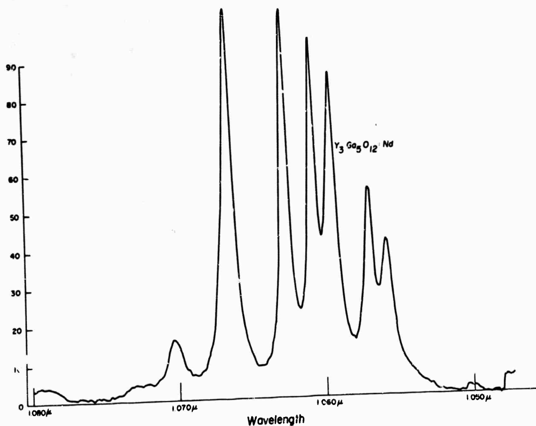
FIG. 2 The spectrum of {}^4F_{3/2} \rightarrow {}^4I_{11/2} fluorescent transitions of the \text{Nd}^{3+} ion in \text{Y}_3\text{Ga}_5\text{O}_{12} measured at room temperature.
