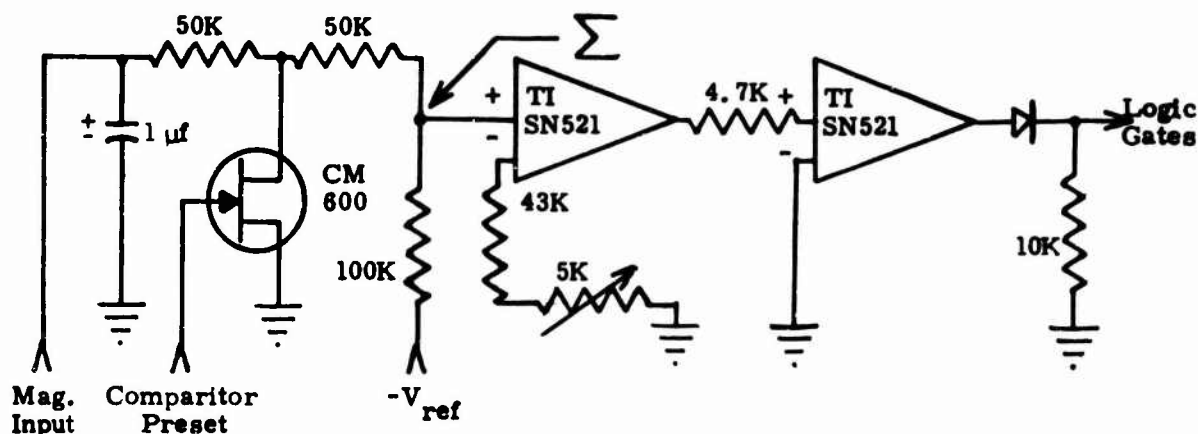
FIGURE 1-12. CHANNEL COMPARITOR
