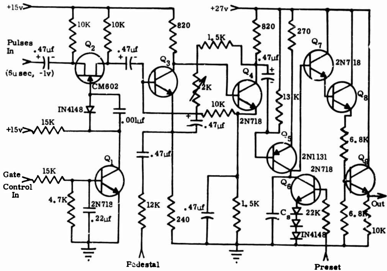
FIGURE 3 - 6. PULSE INTEGRATOR
