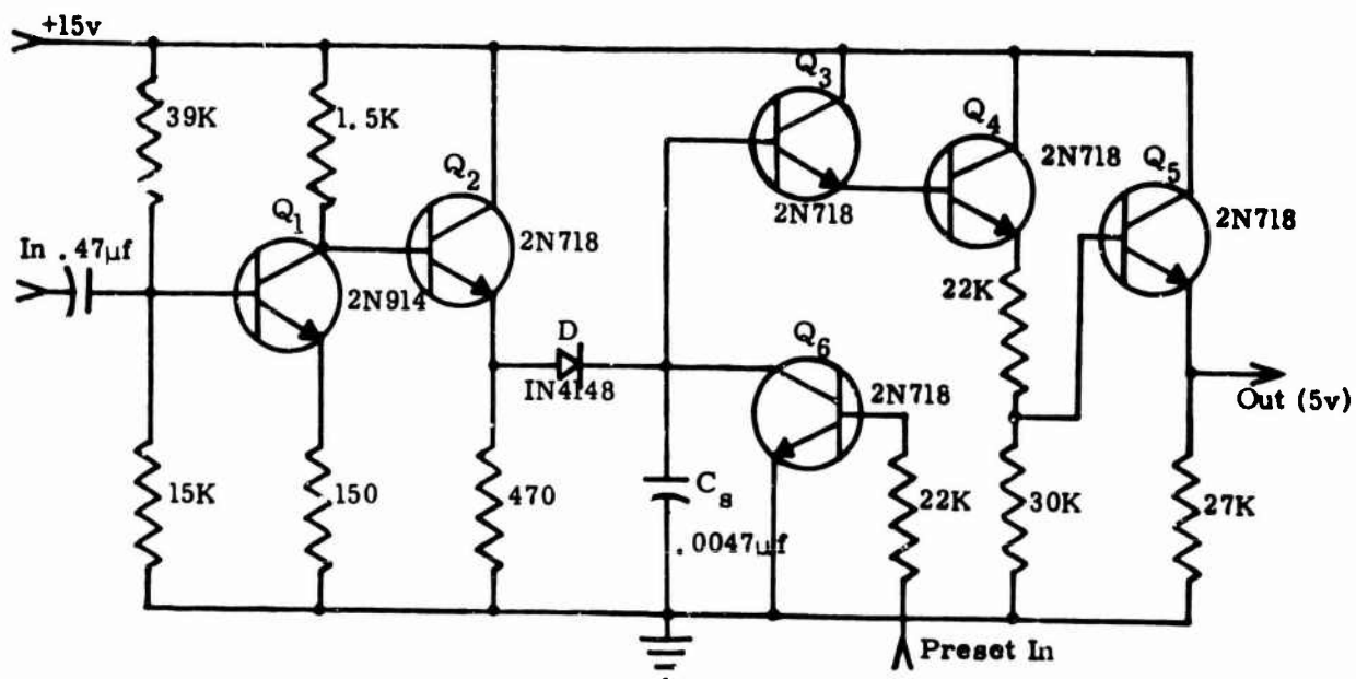
FIGURE 3 - 7. PEAK DETECTOR
