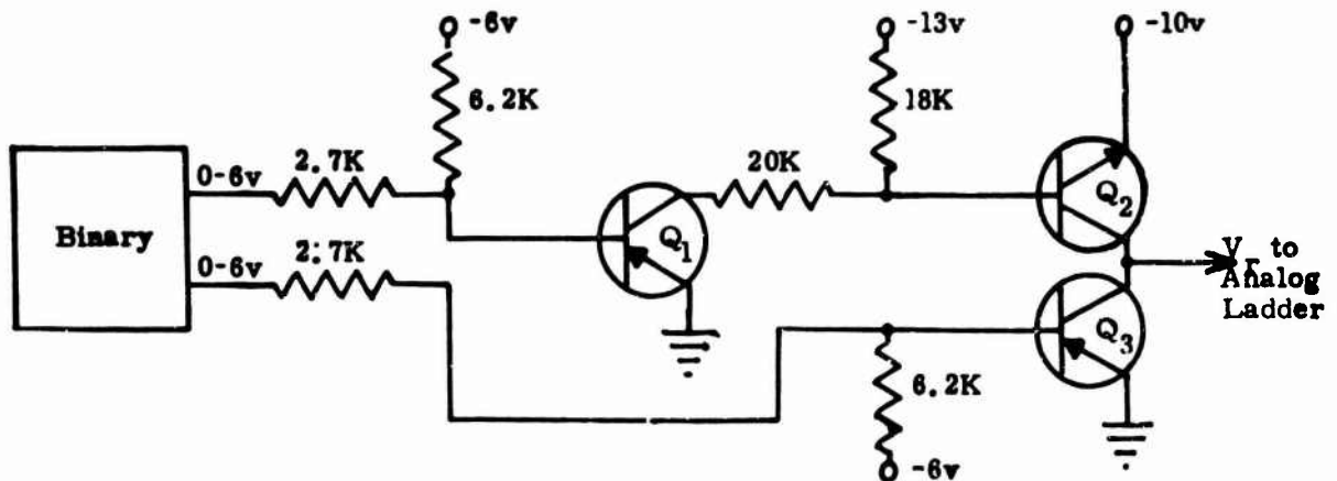
FIGURE 1-14. ANALOG GATE
