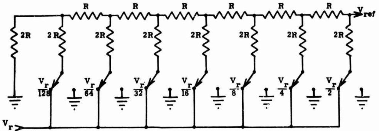
FIGURE 1-13. ANALOG LADDER
