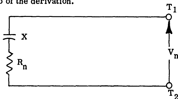
Figure 3. Series equivalent noise circuit
