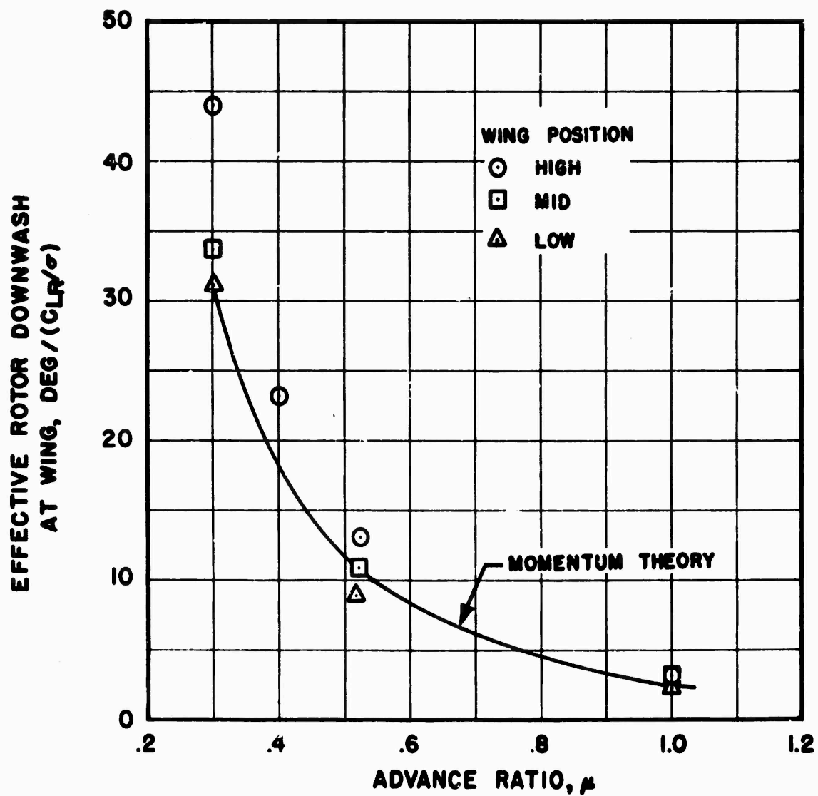
FIGURE 3. EFFECT OF FORWARD SPEED ON EFFECTIVE ROTOR DOWNWASH ANGLE.
