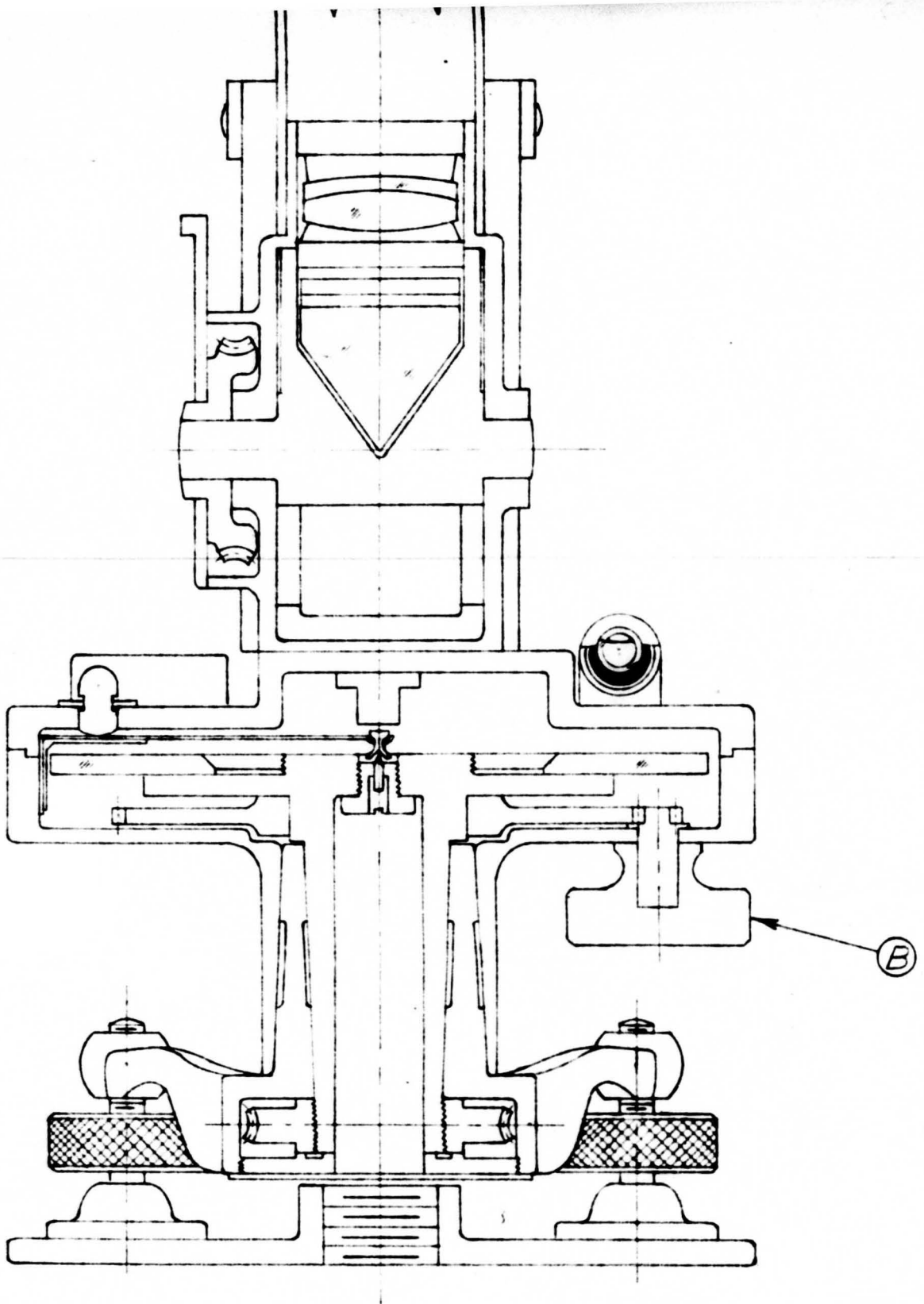
— Section 2-2 —
