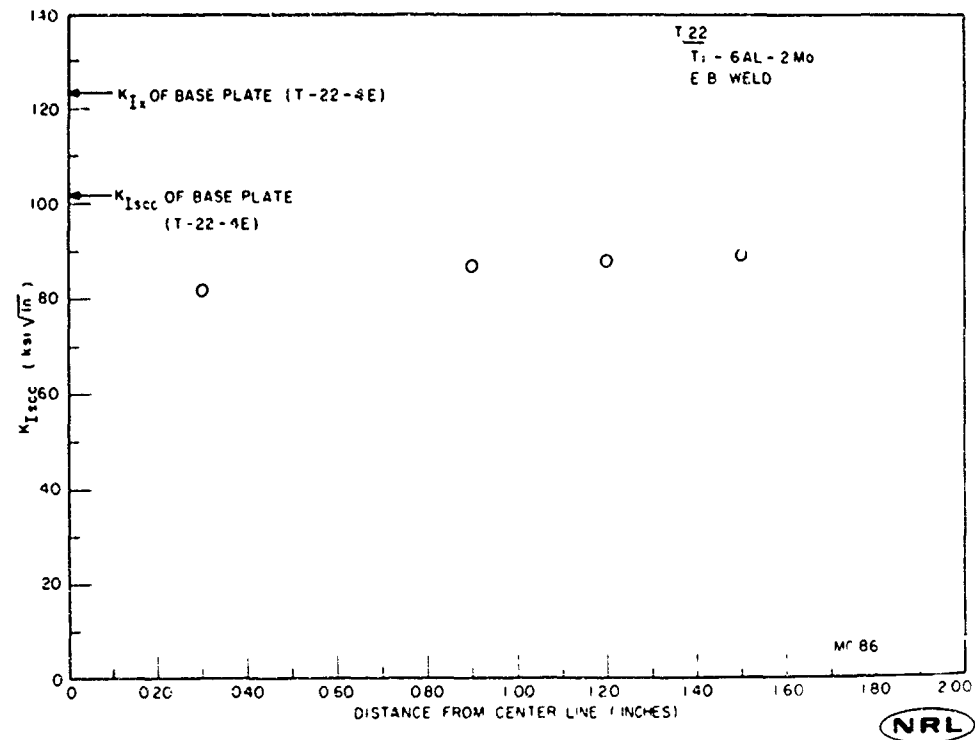
Fig. 77 - Environmental cracking characteristics of an electron beam weldment of titanium alloy T-22
