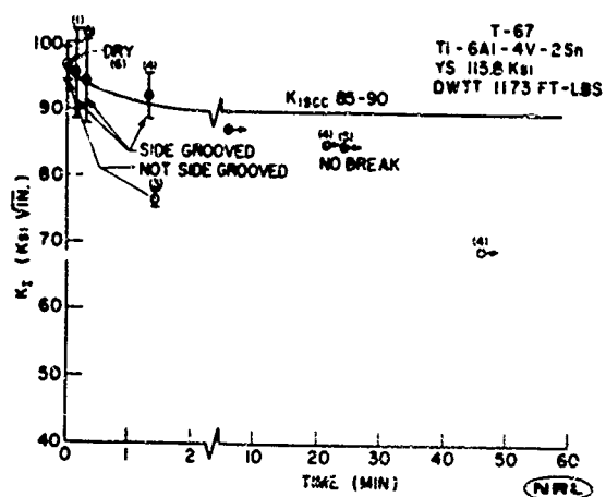
Fig. 33 - Environmental cracking characterization curve for titanium alloy T-67
