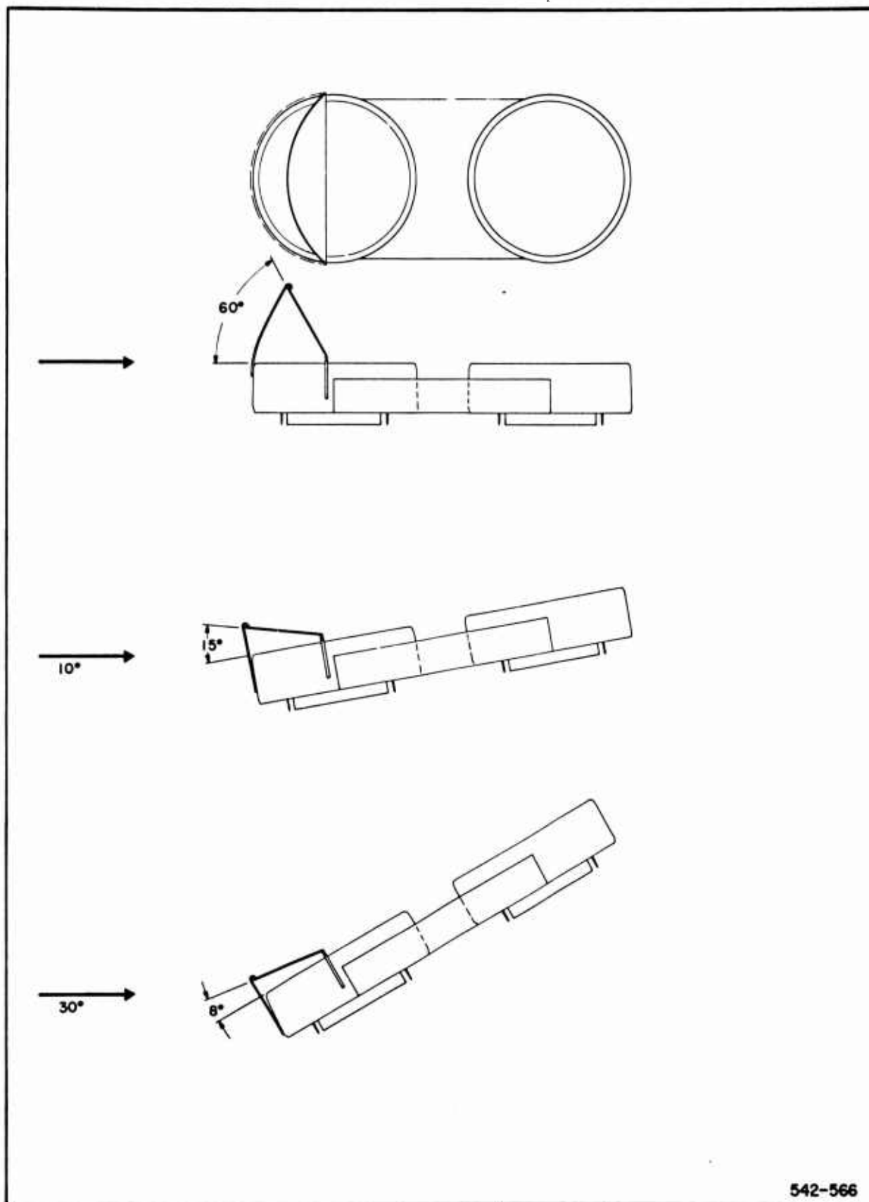
Figure 35. Schematic Drawing of Model in Several Attitudes with a Flap Trim Device
