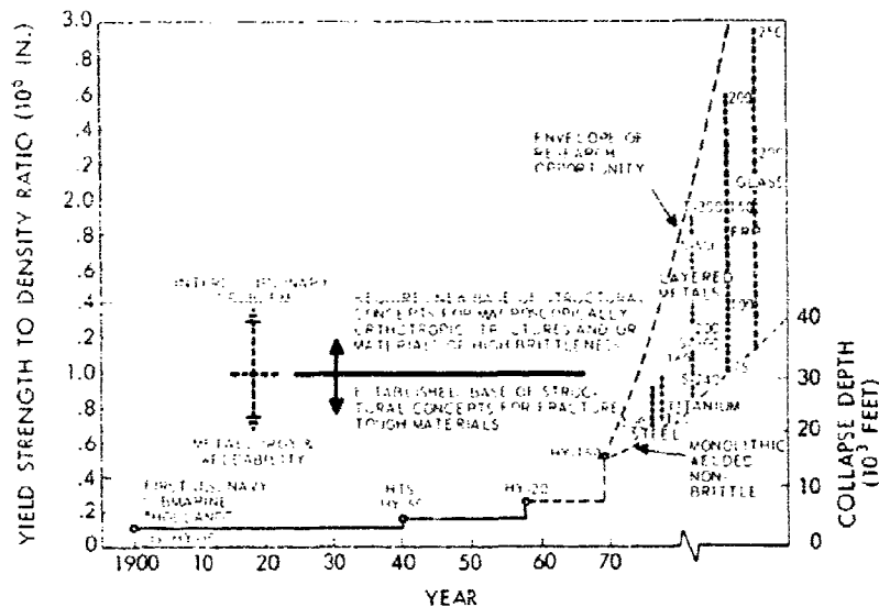
Figure 5.10. Evolutionary and Future Projections of Relative Structural Efficiency of Submarine Hull Structures
