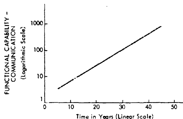
Figure 3.1. Typical Functional Capability of Time History (Semilog Plot)
