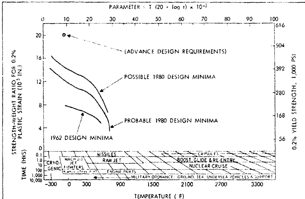
Figure 5.9. Low and Medium Alloy, Ultra-High-Strength Steels
