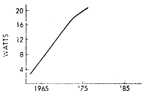
Figure 4.7. Coherent Radiation CW Power (Argon Ion Laser)
