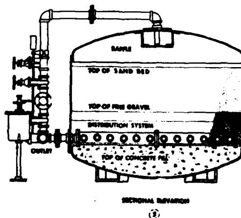
Figure 5-4.—Cross-section of vertical-pressure type water filters
