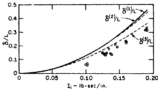
IMPULSE VERSUS CENTRAL DEFLECTION — PINNED (PS) C.R. 1018 STEEL
