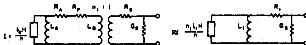
(b) INDUCTIVE
