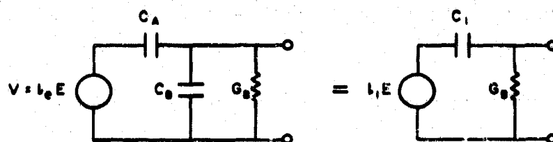
(a) CAPACITIVE
