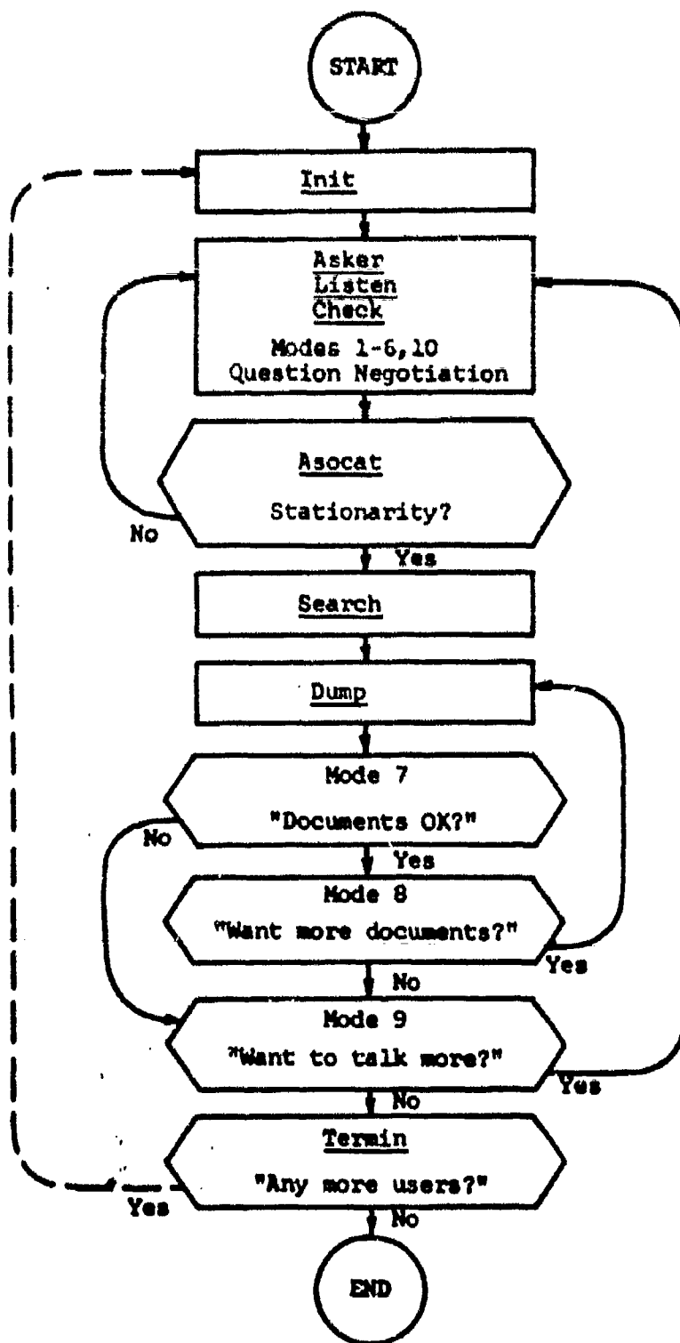
Figure 13. Simplified Diagram of Negotiation Sequence
