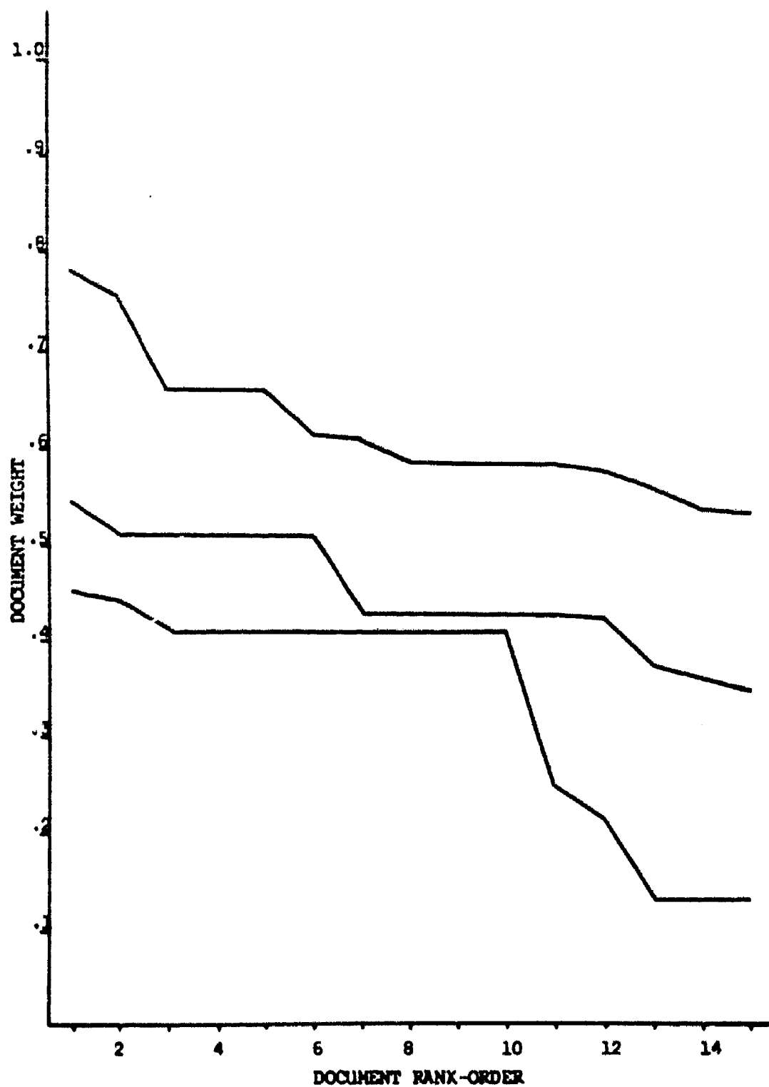
Figure 12. Distribution of Document Weights for Three Searches of the C I S Collection
