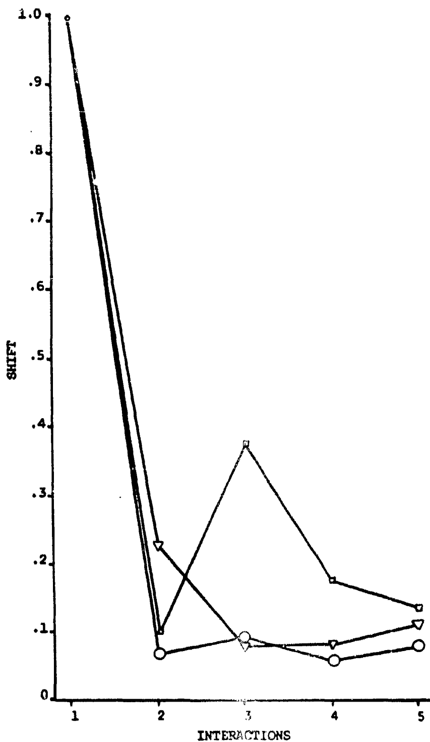
Figure 7. The Shift of the User's Expressed Interest as a Function of the Number of Interactions for Three Negotiations
