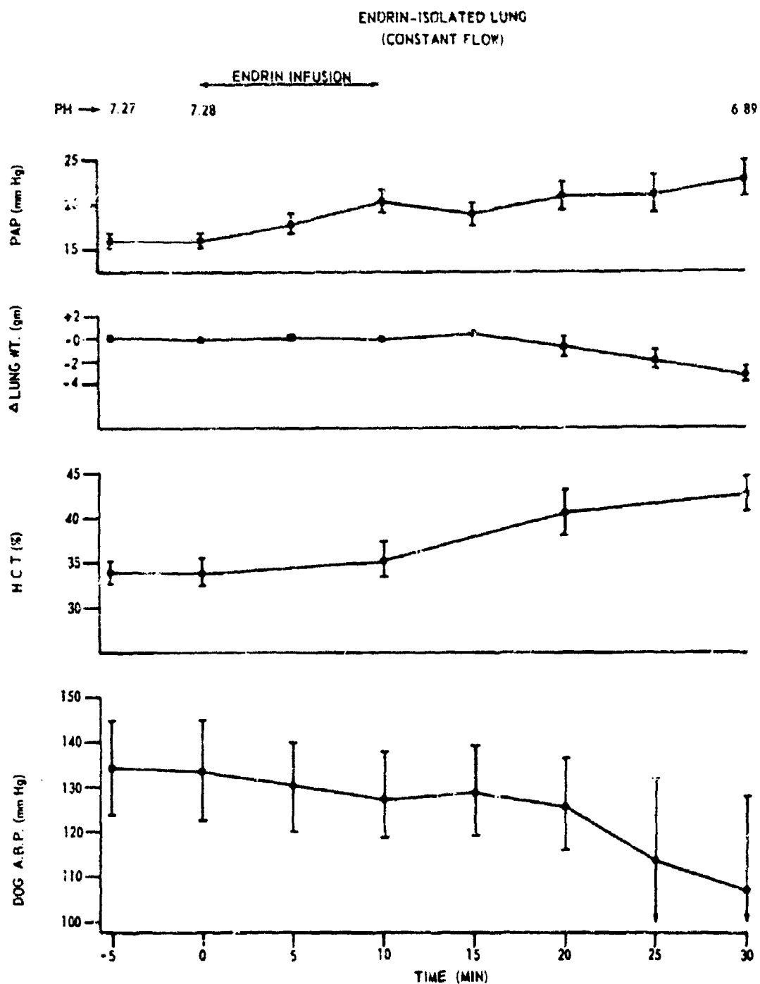
FIGURE 2. Mean values \pm standard errors from five dog pump-perfused isolated lung experiments in which endrin was infused are shown. Dog A.B.P. = table dogs mean systemic arterial blood pressure; Hct = blood hematocrit; \Delta lung wt = change in isolated lung weight from control; PAP = pulmonary artery pressure. Pulmonary blood flow was constant. Endrin infusion began at zero time.
