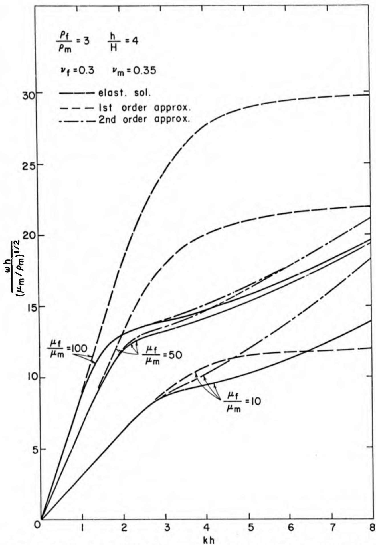
Fig. 2 Lowest longitudinal mode according to effective double stiffness theory
