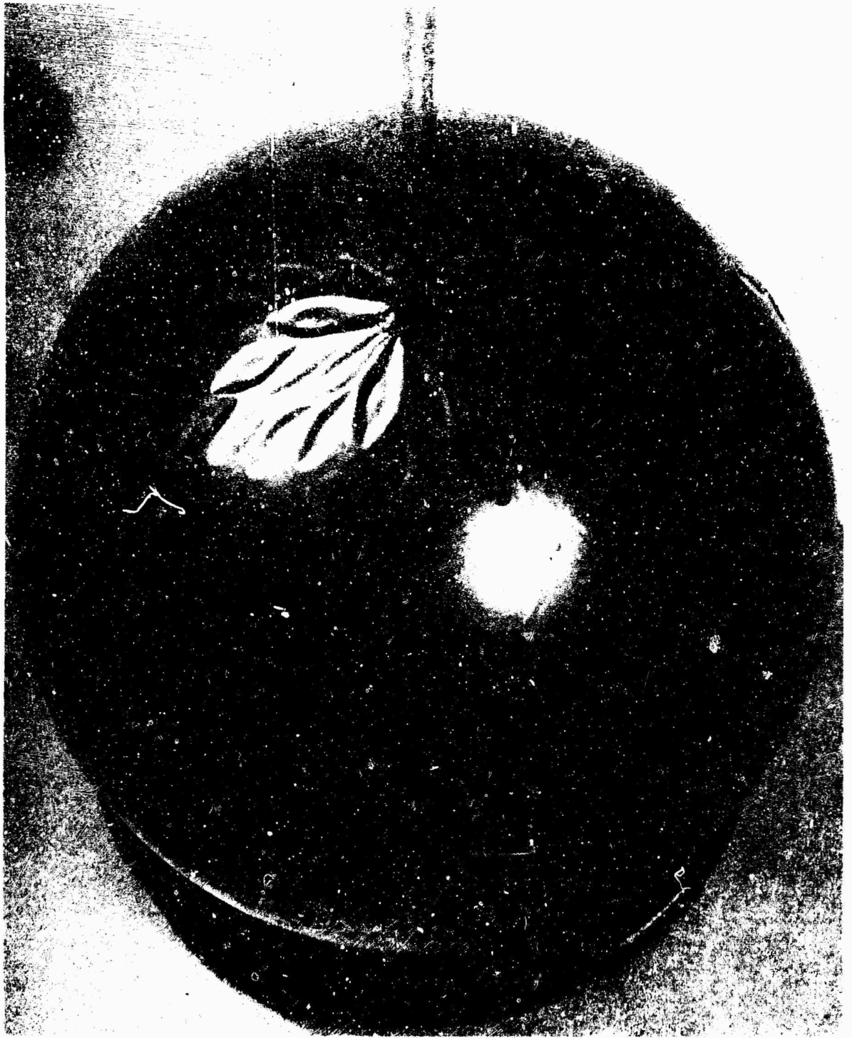
Fig. 23(a)--Buckle Pattern -- Normal Tension Force.
