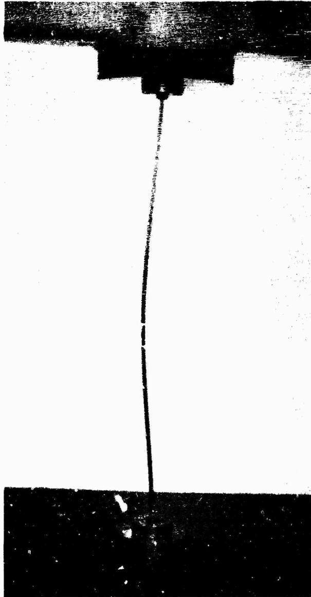
Fig. 2--Typical Euler Buckling of a Long Column With Both Ends Built-In.
