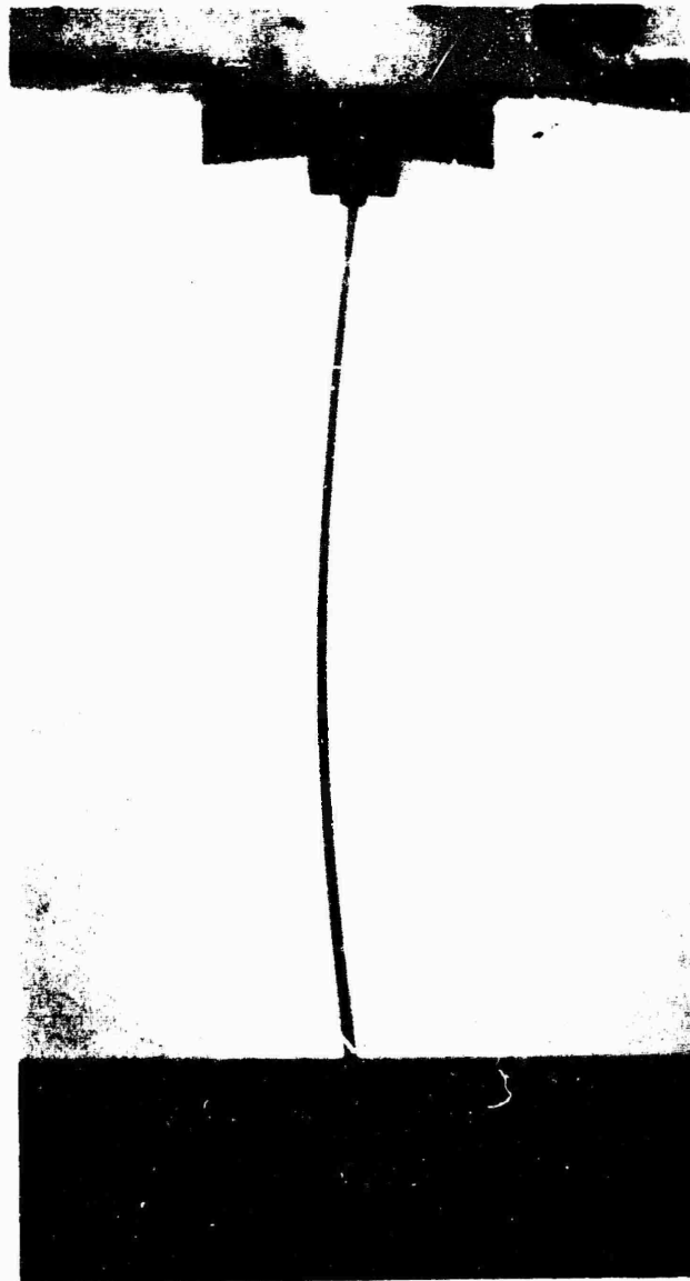
Fig. 1--Typical Euler Buckling of a Long Column With Both Ends Pinned.
