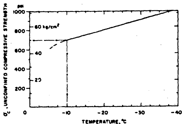
Figure 1. Unconfined compressive strength vs temperature for clear lake ice (from Butkovich, 1964).
