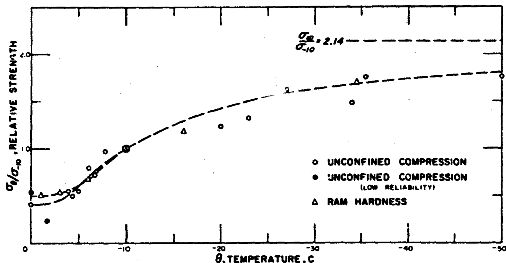
Figure 8. Relative unconfined compressive strength vs temperature (from Mellor-J.H. Smith, 1966).
