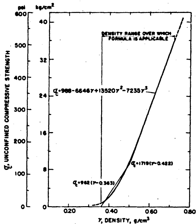
Figure 4. Linear unconfined compressive strength vs density relationships for the combined Butkovich and J. L. Smith data above and below the transition density of 0.50 \text{ g/cm}^3 in relation to the polynomial relationship for the entire data range. Snow temperature -10\text{C} .
