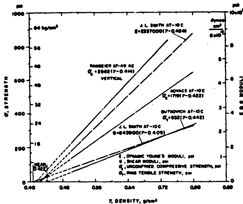
Figure 9. Intercept density relationship between the extended straight-line portions of different tests.
