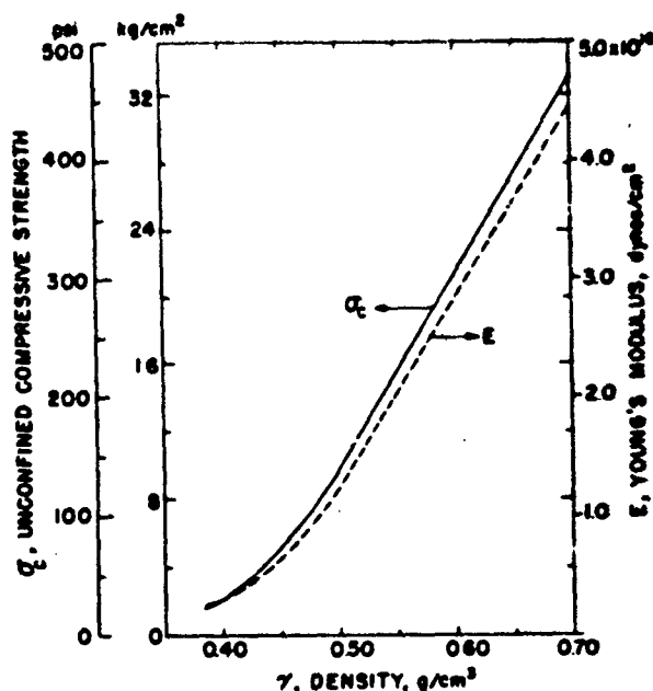
Figure 5. Curve trend comparison between equation 11's unconfined compressive strength relationship and J. L. Smith's dynamic Young's modulus vs density relationship. Snow temperature -10C.
