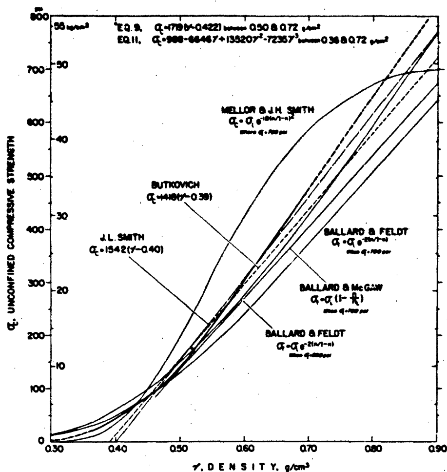
Figure 6. Comparison of the unconfined compressive strength vs density relationship of eq 11 with earlier relationships. Snow temperature -10C.
