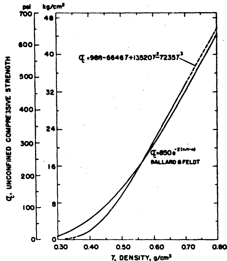
Figure 7. Comparison between the Ballard-Feldt and eq 11 unconfined compressive strength vs density relationships. Snow temperature -10^{\circ}\text{C} .
