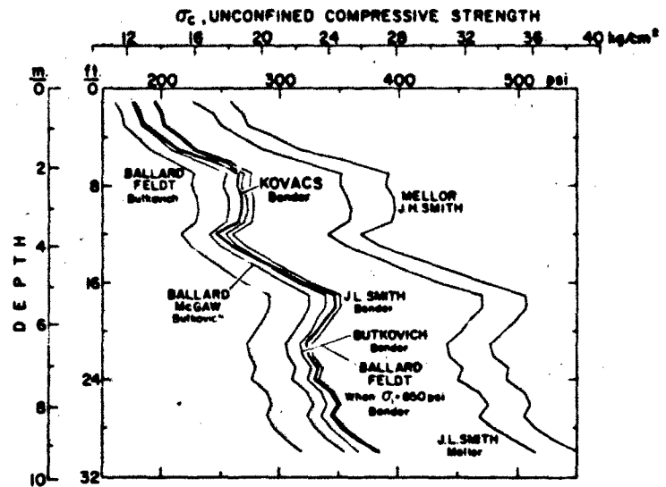
Figure 10. Relationship between values obtained from the different unconfined compressive strength equations when they are used to determine strengths from depth-density and temperature profiles. The name of the investigator who developed the equation is shown in capital letters; other names indicate type of temperature correction used.
