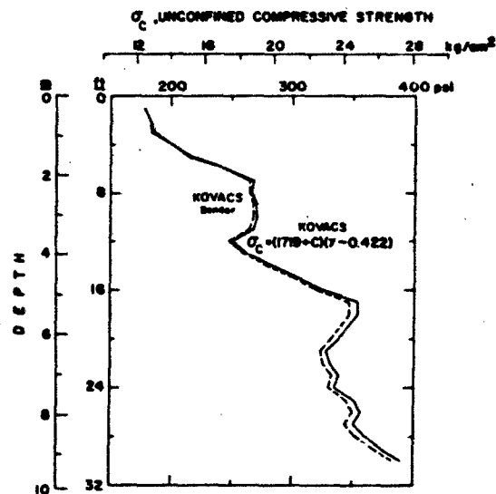
Figure 11. Comparison between the values obtained from eq 9, temperature-corrected after Bender (eq 12), and from eq 14 when they are used to determine the unconfined compressive strength of polar snow from depth-density and temperature profiles.
