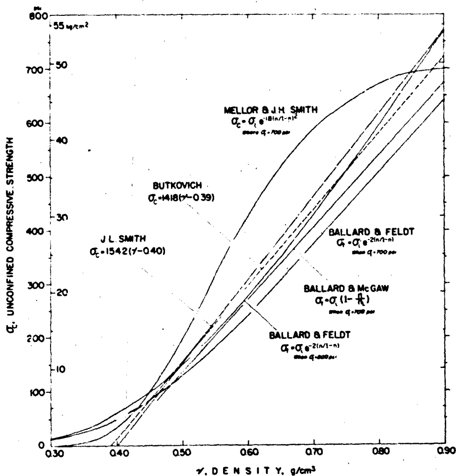
Figure 2. Comparison of existing unconfined compressive strength vs density relationships for polar snow at -10°C.
