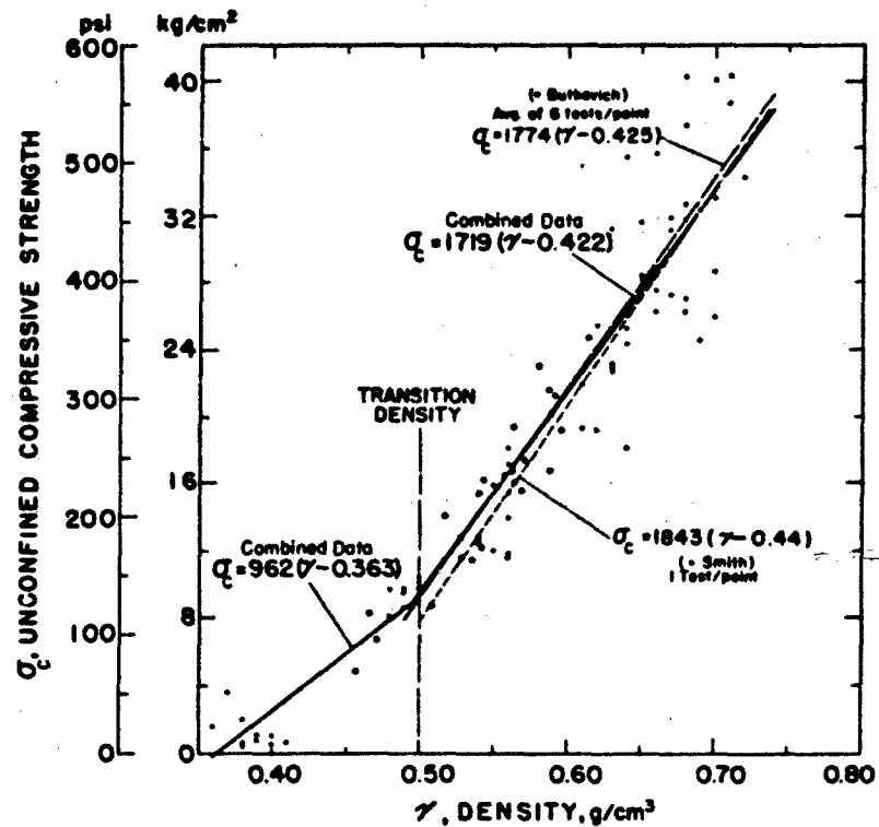
Figure 3. Linear relationships of unconfined compressive strength vs density for data of Butkovich and J. L. Smith above and below the transition density of 0.50 g/cm 3 . Snow temperature -10C.
