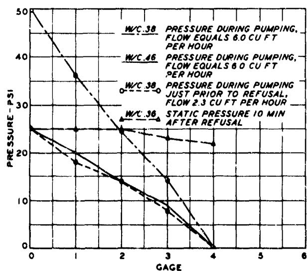
Fig. 11. Pressure gradient during and after grouting 0.03-in. crack, neat cement + Intrusion Aid grout
