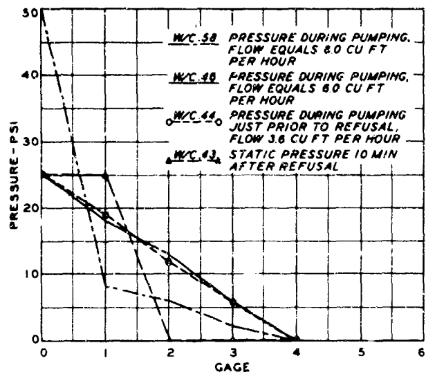
Fig. 7. Pressure gradient during and after grouting 0.03-in. crack, neat grout
