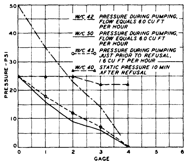
Fig. 9. Pressure gradient during and after grouting 0.03-in. crack, 1 cement:1 fly ash grout
