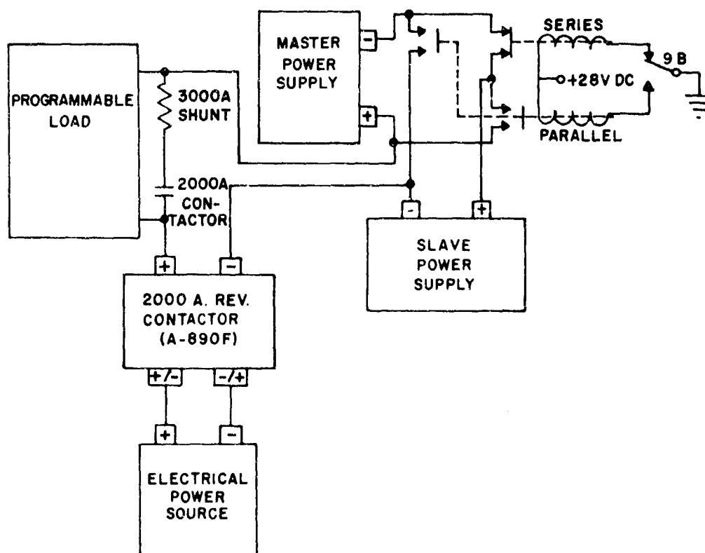
Fig. 4. High-current circuit.
