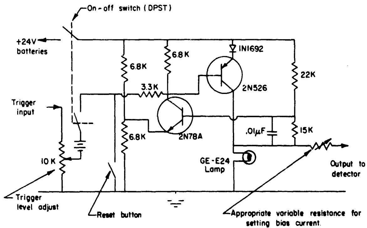
Figure 2.2 Detector current supply. A trigger pulse to the circuit will interrupt the current (until manually reset).
