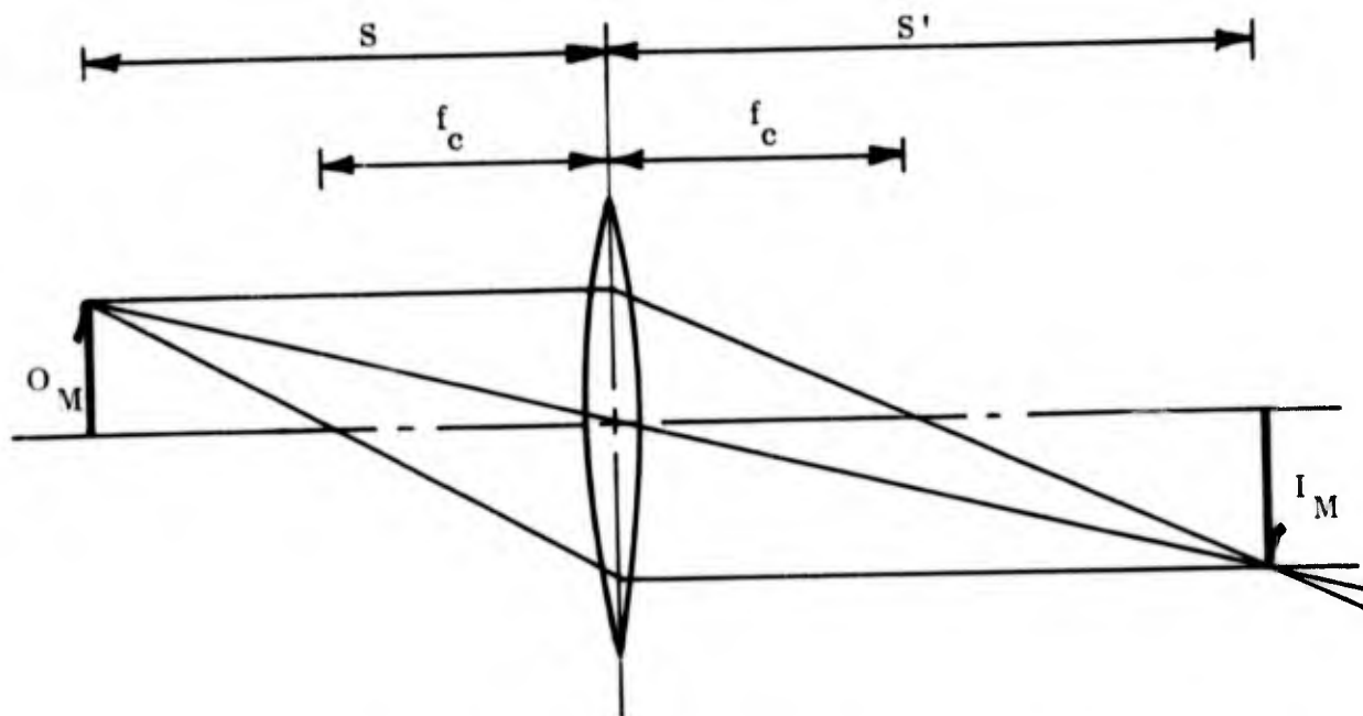
Graphical Representation of a Complex Lens System
