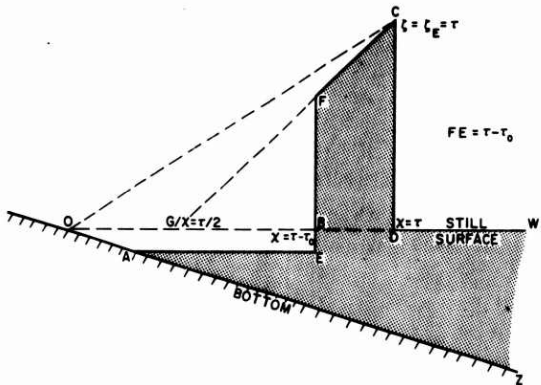
Figure 3 Finite duration step-pressure response
