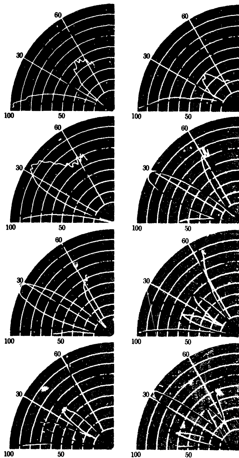
Figure 27. Vertical patterns of Figure cage with cage feed open (solid) and short-circuited (dashed).
