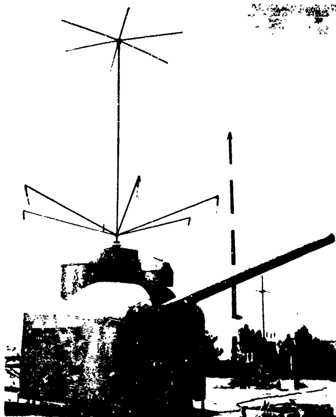
Figure 1. DISCAGE antenna on 5-inch, 54-calibre gun turret.
