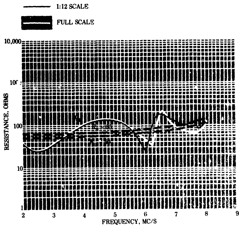
Figure 15. Measured input resistance of the cage section with the disccone terminated in the high-pass filter (termination effects simulated by coaxial stubs during model studies). Dashed curves show variations of R_{\pi k} for two values of R_0 .
