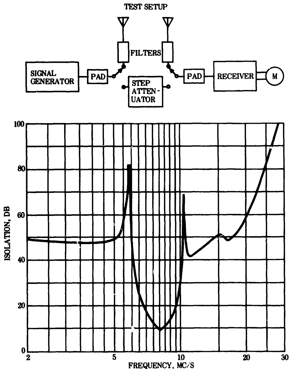
Figure 22. Measured isolation between cage and disccone sections with auxiliary filters installed.
