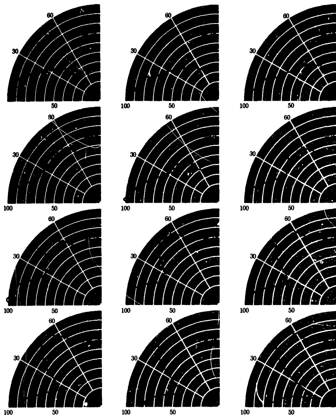
Figure 25. Vertical patterns of cage at high end of operating band with discone feed open (1:24 model).
