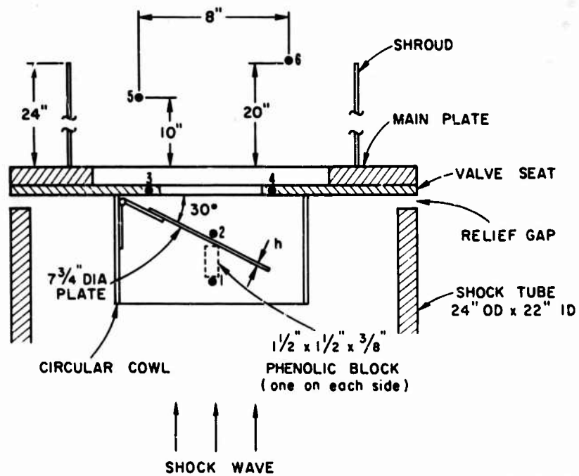
FIG. 4 SWING-VALVE SET-UP
