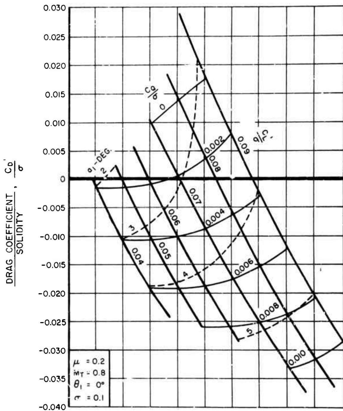
Figure 2. Calculated Characteristics of a Rotor With 0^\circ Twist for \mu = 0.2 and M_T = 0.8 .
