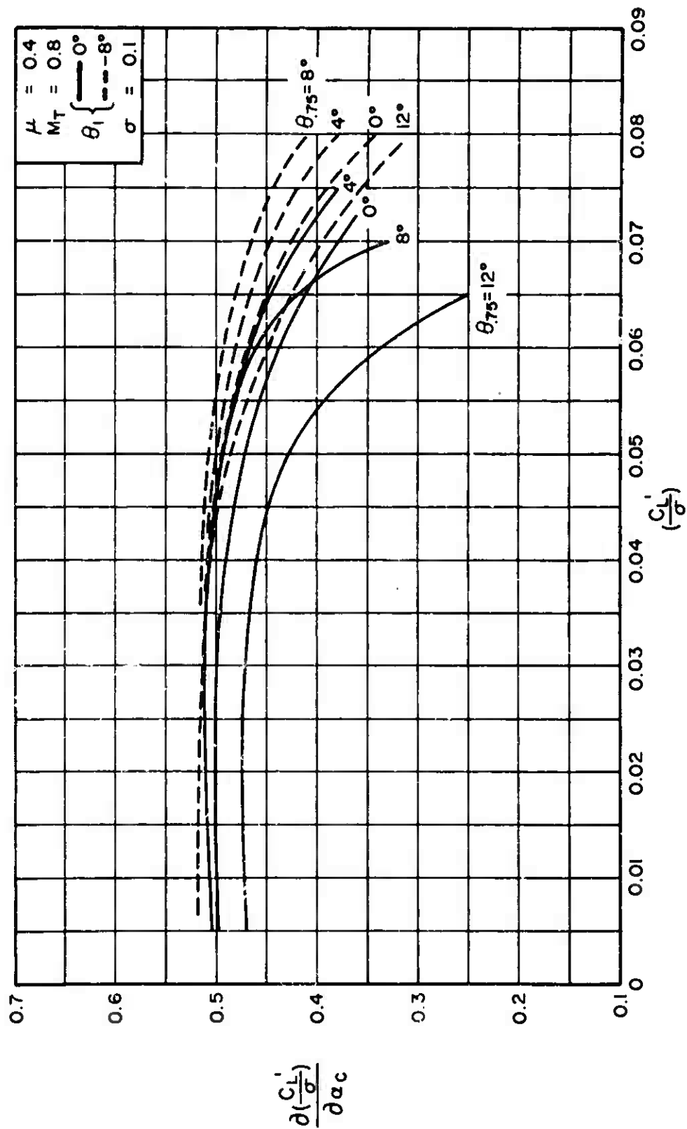
Figure 22. Effect of Blade Twist on \alpha_c Derivatives
