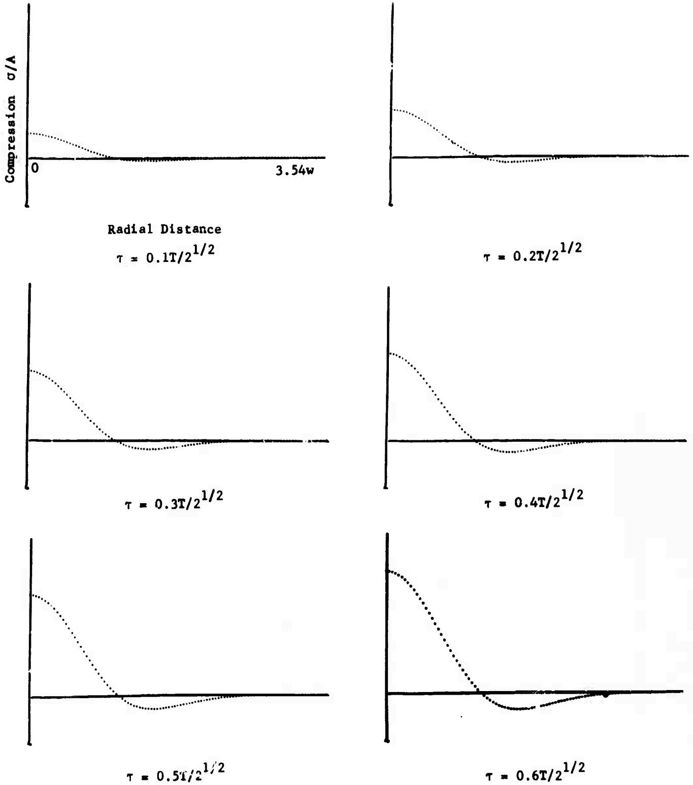
Figure 10. Sound Wave Compression at Various Times After An Initial Impulse
