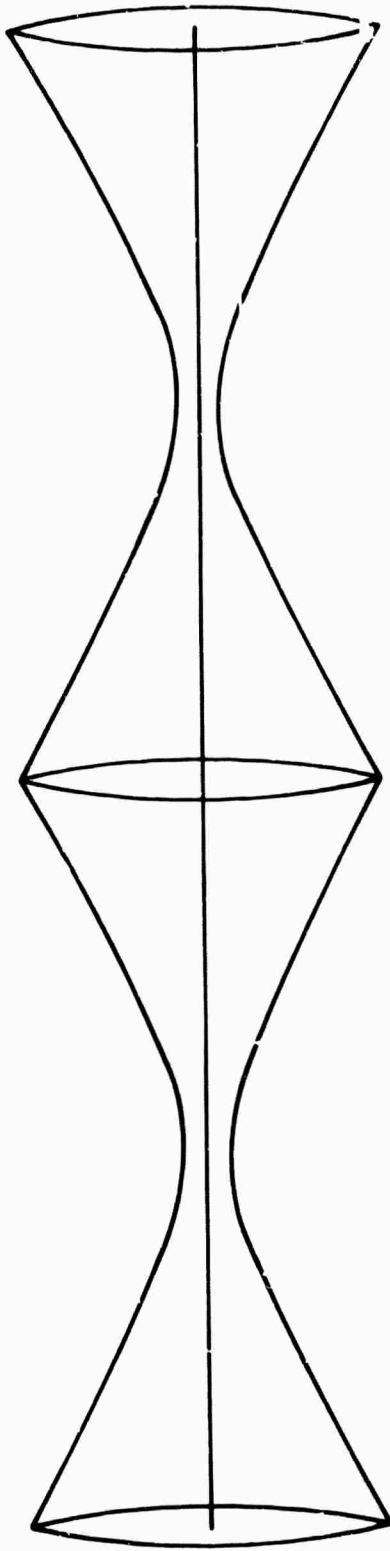
Confocal Mode Propagation in a Sequence of Thin Lenses
