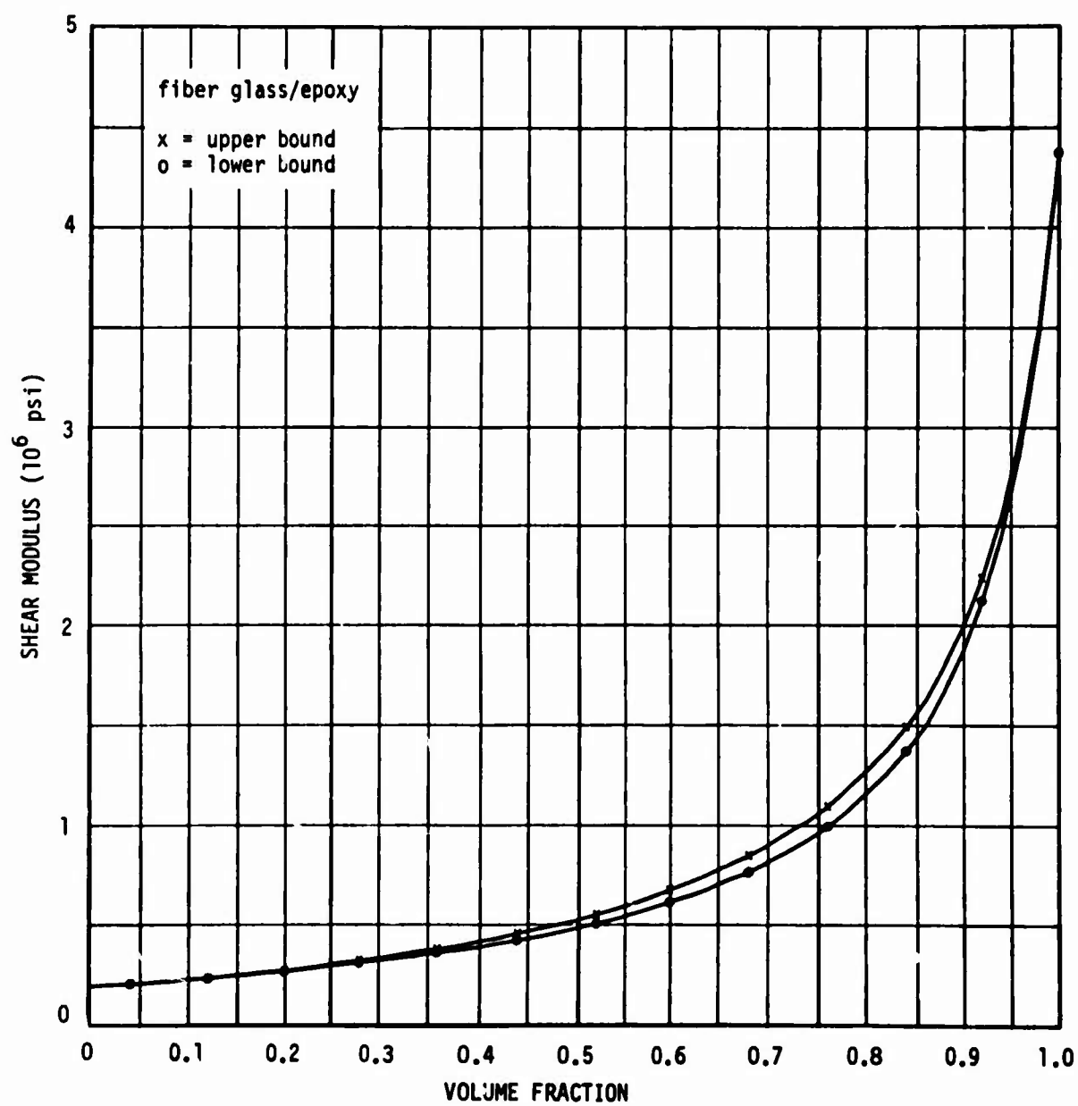
Figure 9. Shear Modulus G_{12}^* vs. Volume Fraction \phi = 45 degrees
