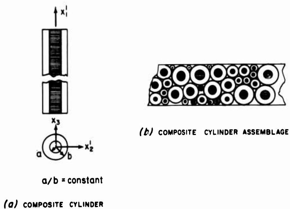
Figure 3. Composite Cylinder Model.
