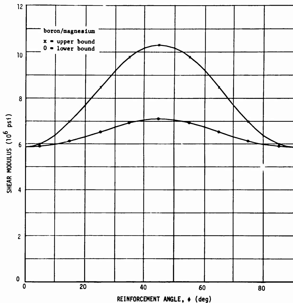
Figure 31. Shear Modulus G_{31}^* vs. Reinforcement Angle Volume Fraction = 0.5
