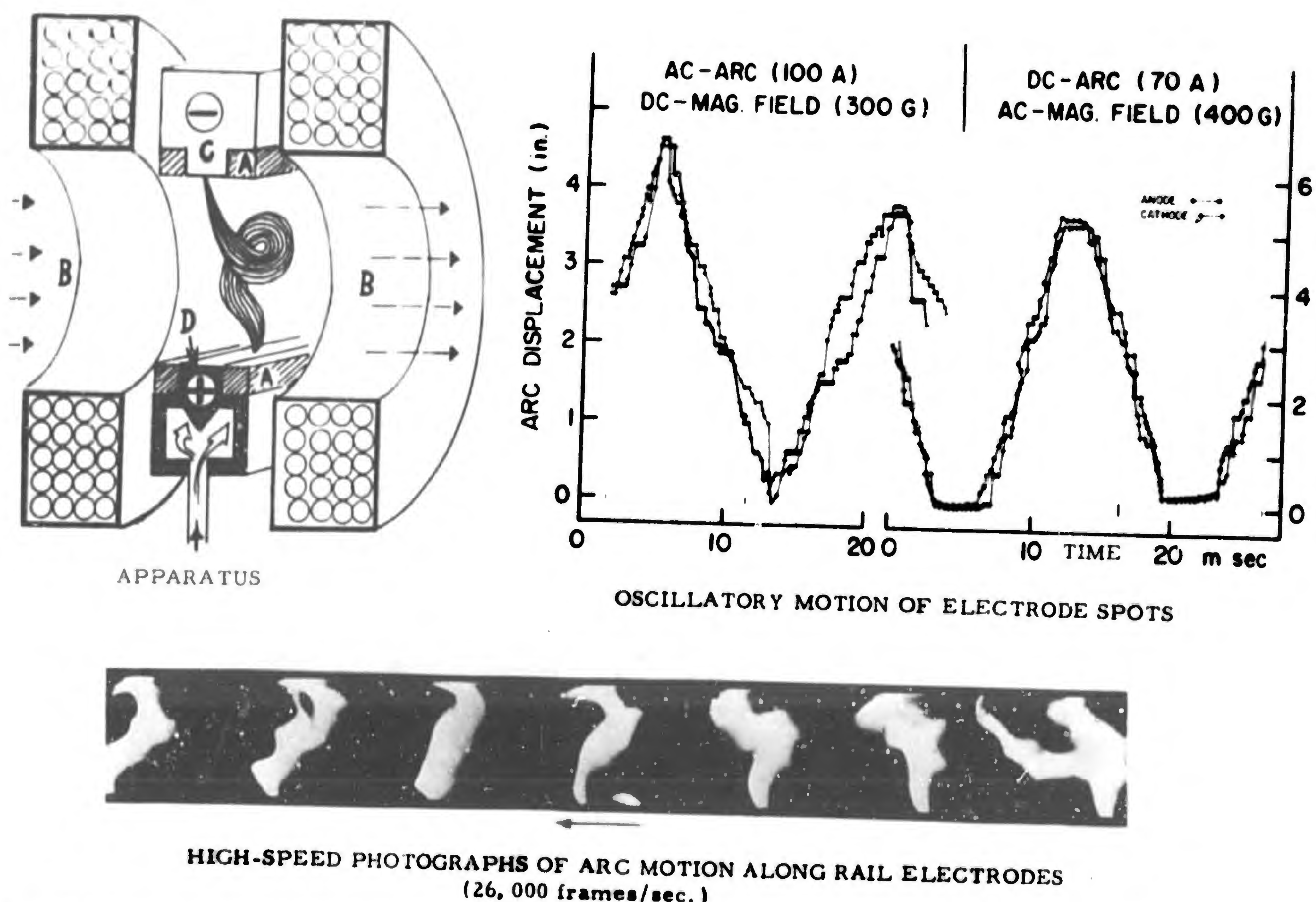
Figure 1. (a) Apparatus; (b) Oscillatory motion of electrode spots; (c) High-speed photographs of arc motion along rail electrodes (26,000 frames/sec).
