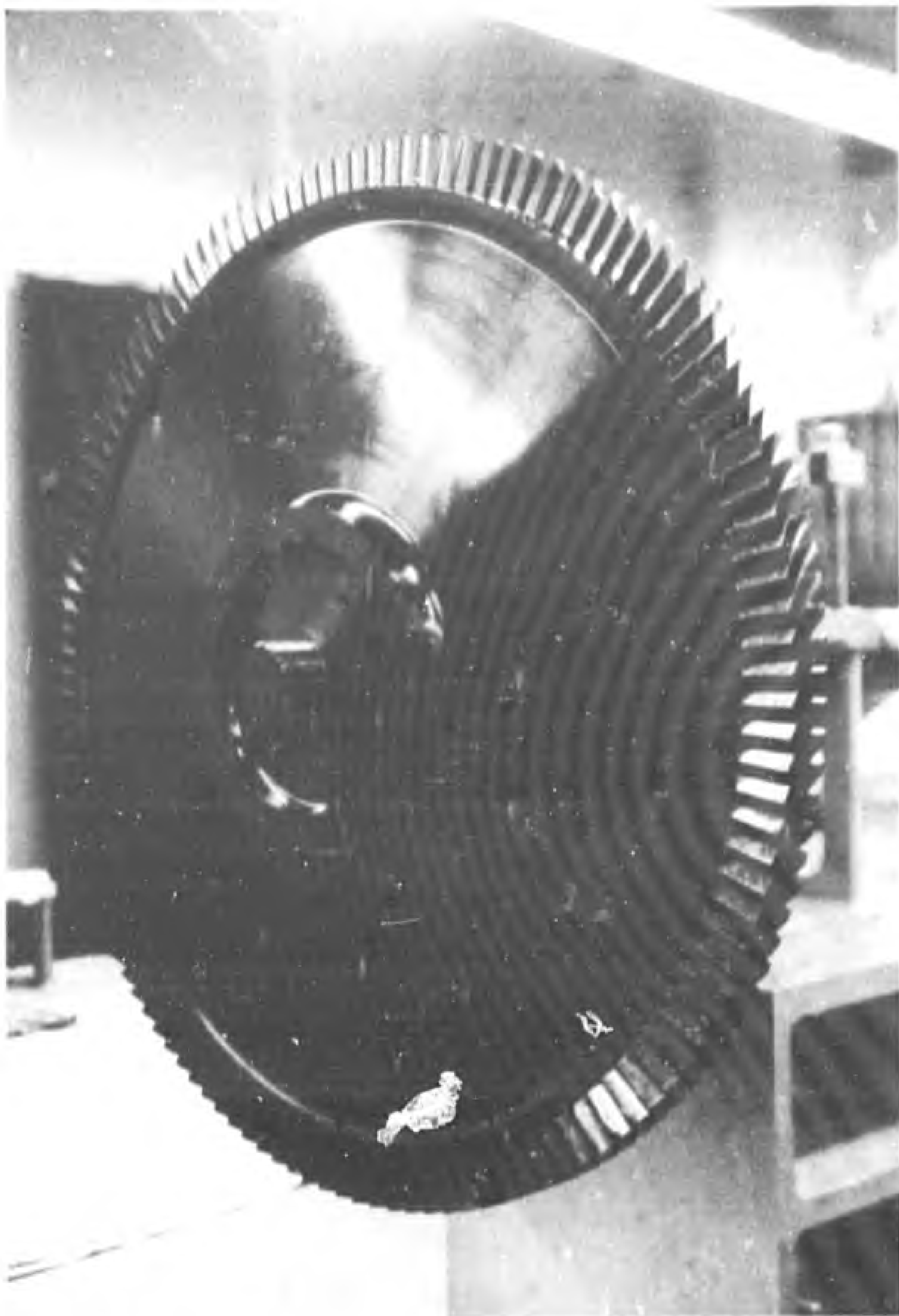
Figure 1. Blunt-trailing-edge supersonic-compressor rotor.
