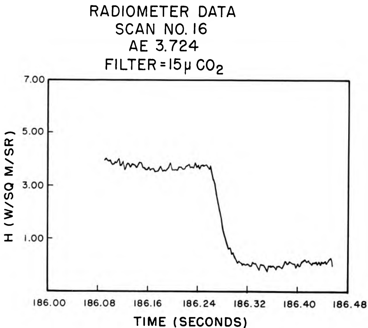
Figure 3. A typical horizon profile taken in the 15\mu carbon-dioxide absorption band.
