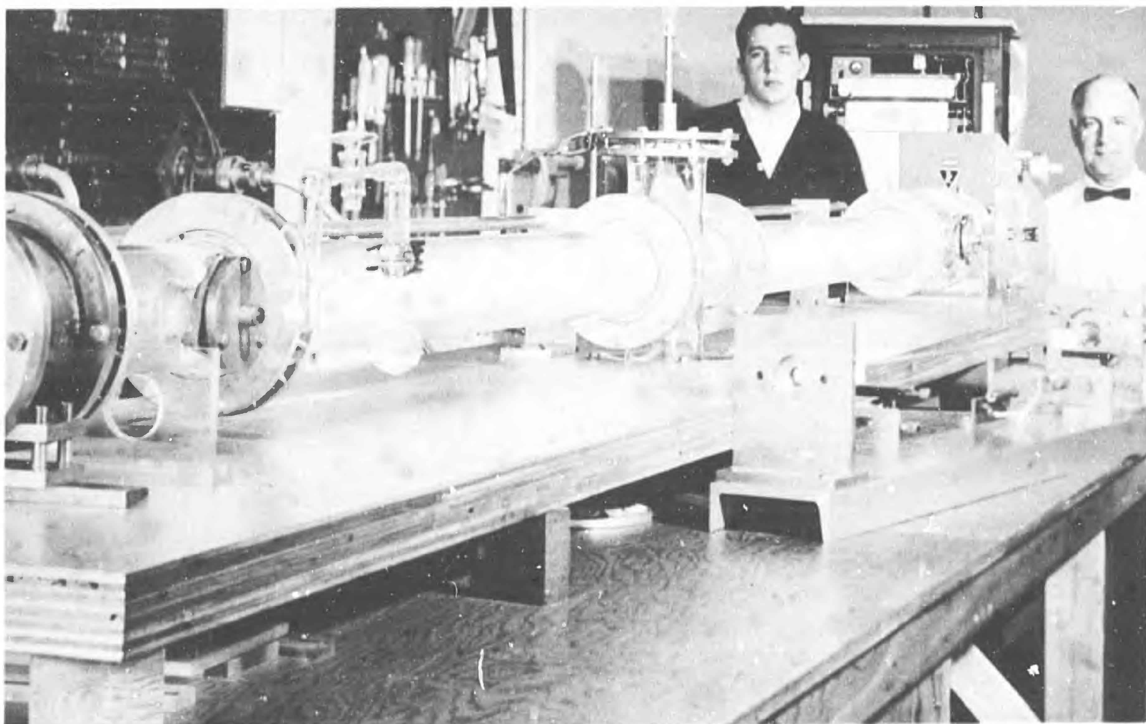
Figure 2. Water-vapor gas laser.
