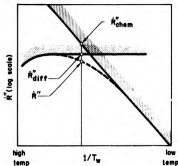
Figure 1. Transition from reaction-rate control to diffusion control on the Arrhenius plane.
