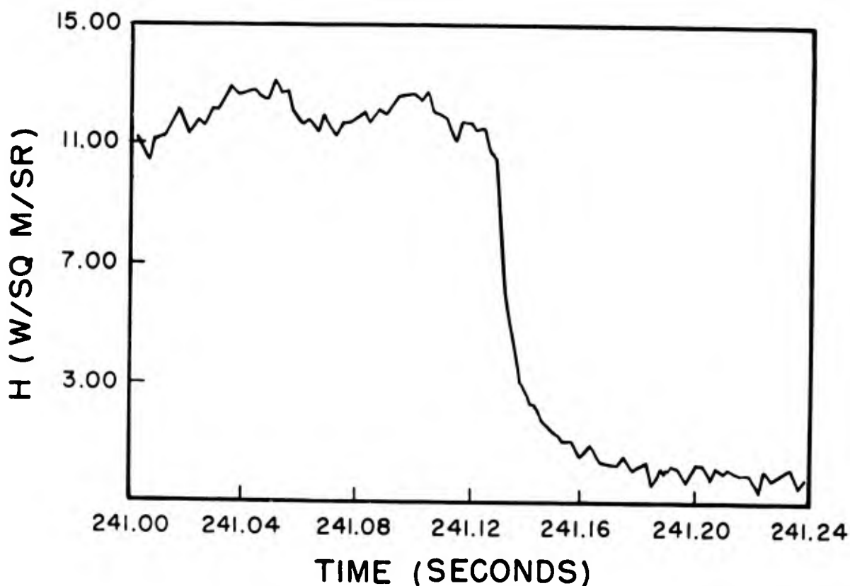
Figure 1. Horizon profile as observed at a wavelength of 19\mu .
