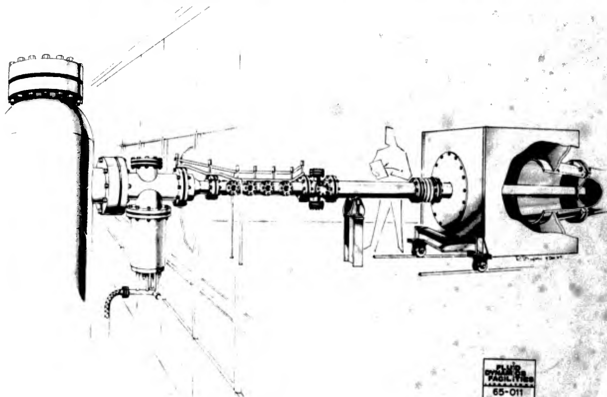
Figure 1. Supersonic-combustion-simulation facility.
