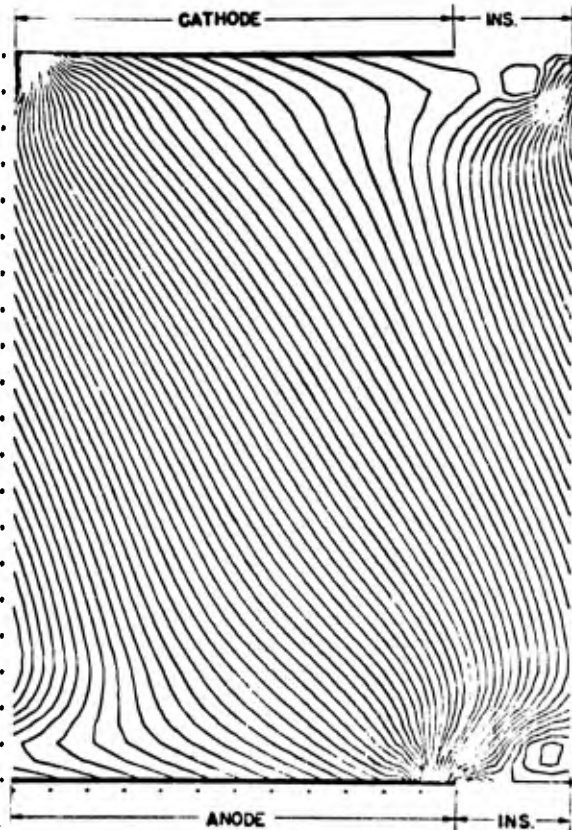
Figure 2. Current streamlines. Boundary layers for the gas temperature ( T_g = 1600 at wall, 3050, 3200, 3030, and 3000^\circ\text{K} in the core) and for the gas velocity ( U = 600 at wall, 2460, 2720, 2880, and 3000 m/sec in the core). Contour interval 100 A/m.
