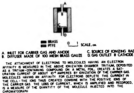
Figure 3. Electron capture ionization detector.
