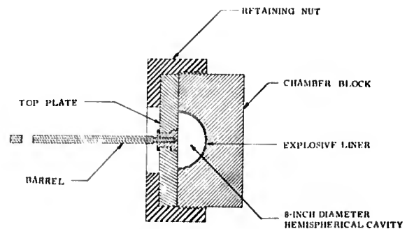
Figure 1. Implosion-driven hypervelocity launcher of the University of Toronto's Institute for Aerospace Studies.
