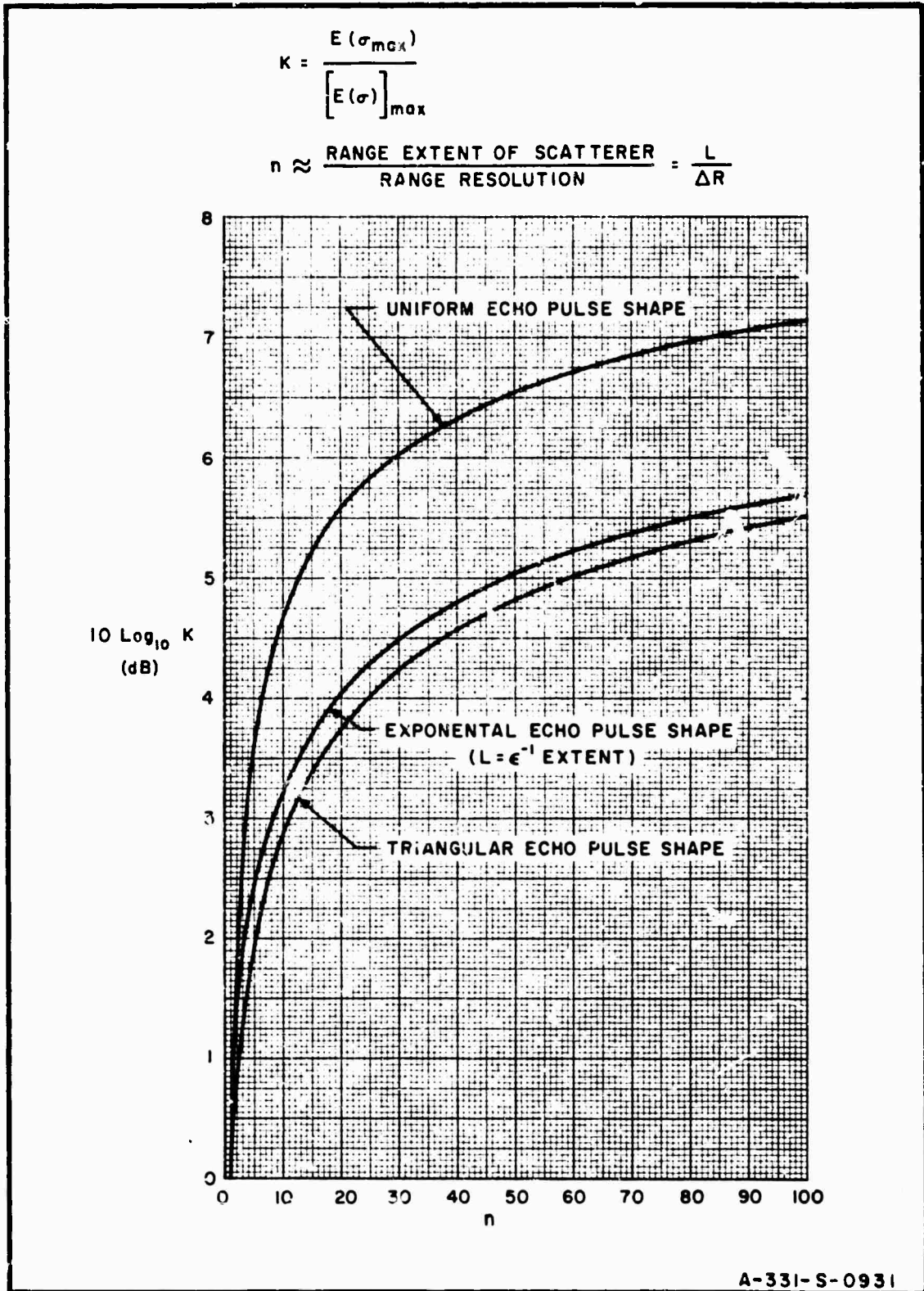
FIG. 3 RATIO OF EXPECTED-PEAK TO PEAK-EXPECTED RCS OF RANDOM DISTRIBUTED SCATTERER
