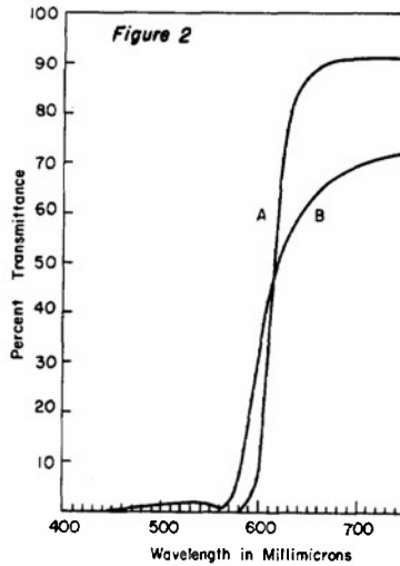
Figure 2 Spectral transmittance of red filter samples A and B
