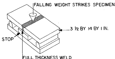
Fig. 5 - Drop-weight test
