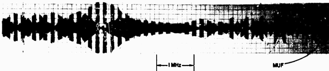
Fig. 15. AMPLITUDE VS FREQUENCY BEHAVIOR OF THE ONE-HOP LOWER RAY DURING ANTENNA-SWITCHING EXPERIMENT.
