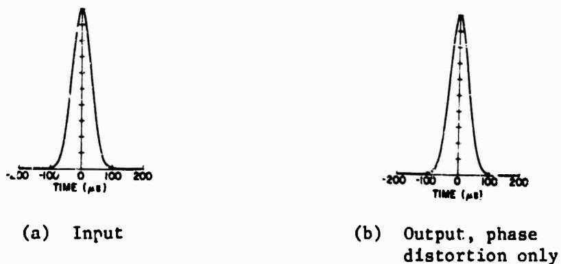
Fig. 37. ENVELOPE SHAPE OF IONOSPHERICALLY PROPAGATED 50 \mu\text{s} , 17.5 MHz PULSES BEFORE AND AFTER IONOSPHERIC PASSAGE.
