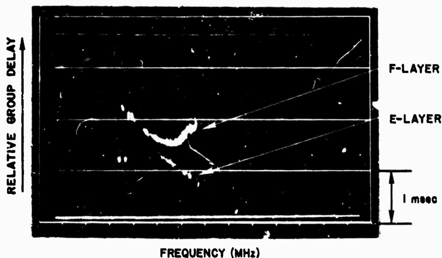
Fig. 47. IONOGRAM MADE DURING MIDDAY TESTS.
