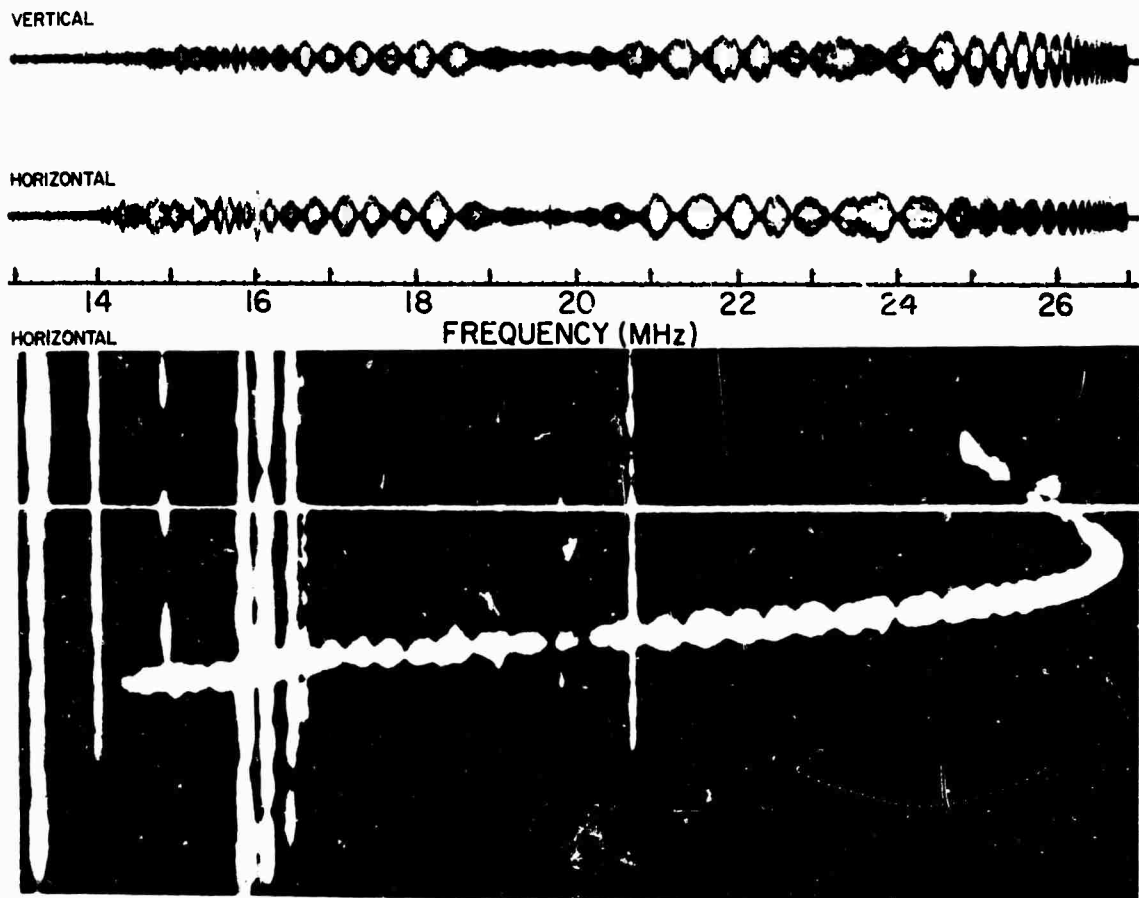
Fig. 17. RESULTS OF THE TWO-RECEIVER EXPERIMENT.
