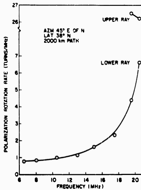
(b) Polarization rotation rate
