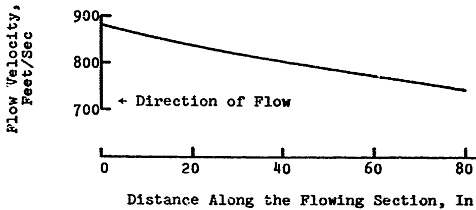
Figure 47 Flow and Reaction Zone Velocities in the Flowing Section, Run 81
