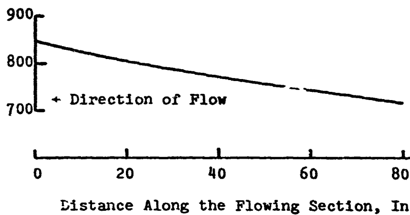
Figure 34 Flow and Reaction Zone Velocities in the Flowing Section, Run 65
