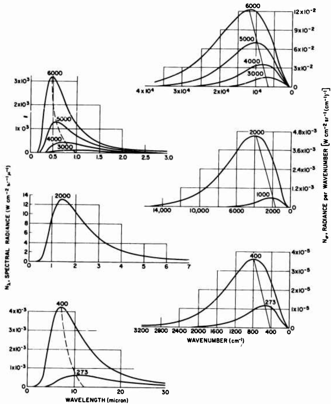
Figure B-3. Spectral radiance N_\lambda and radiance per reciprocal centimeter N_\sigma of blackbodies at various temperatures (°K) plotted on arithmetic scales; note values given are per square centimeter of surface and must be multiplied by 10^4 to obtain values in \text{W m}^{-2} \text{sr}^{-1} \mu^{-1} or \text{W m}^{-2} \text{sr}^{-1} (\text{cm}^{-1})^{-1} . The dashed and diagonal lines show Wien's displacement law. Figure by P.R. Gast.
