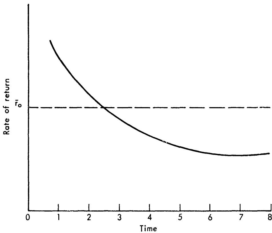
Fig. 11—Autocorrelated earnings
