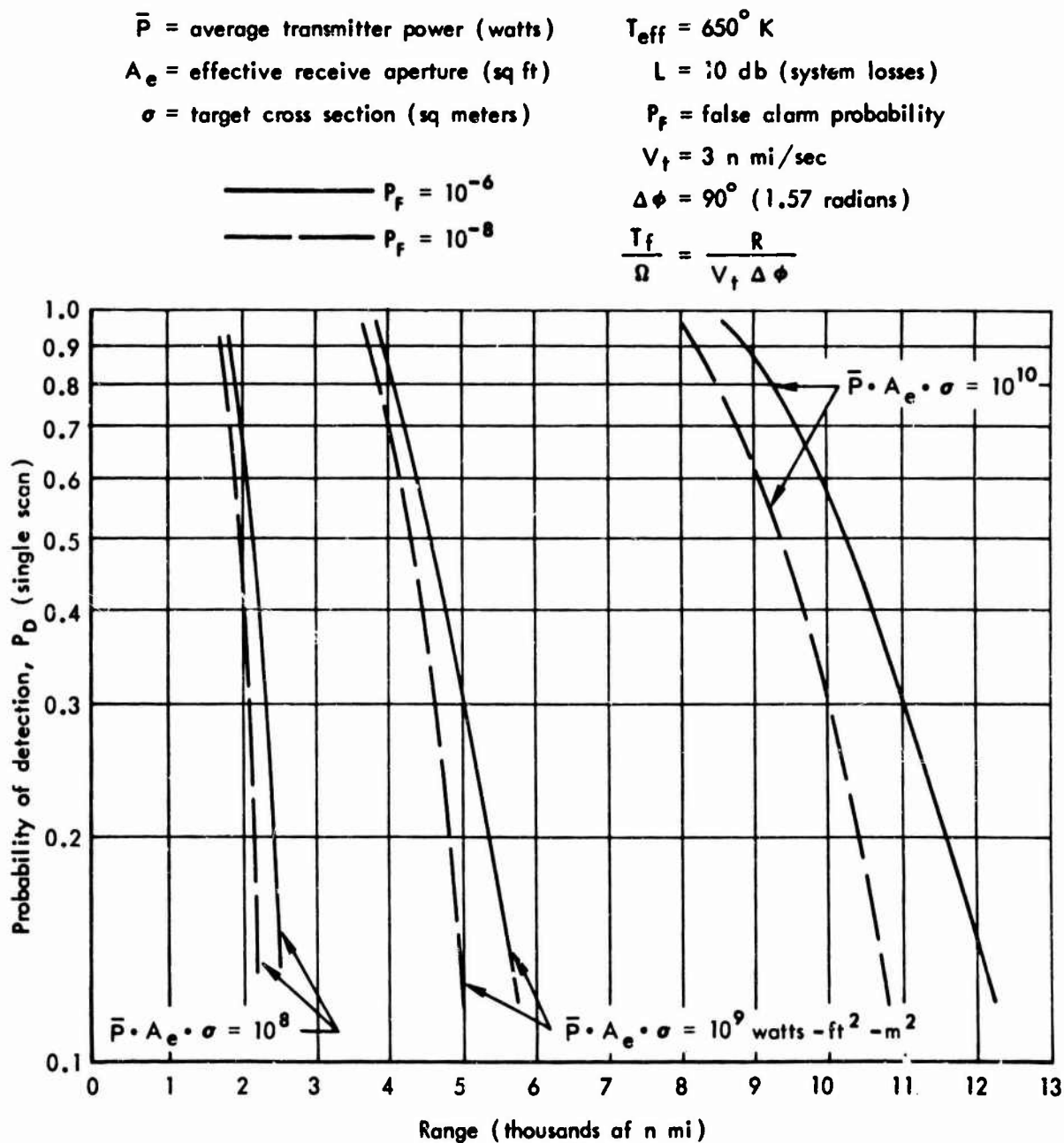
Fig. 4--Detection probability versus range on a single scan
