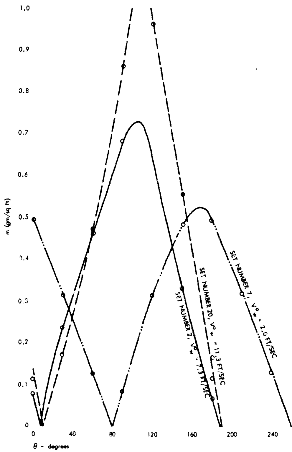
Figure 3 VARIATION OF PLATE COLLECTOR DEPOSITS WITH PLATE ANGLE
