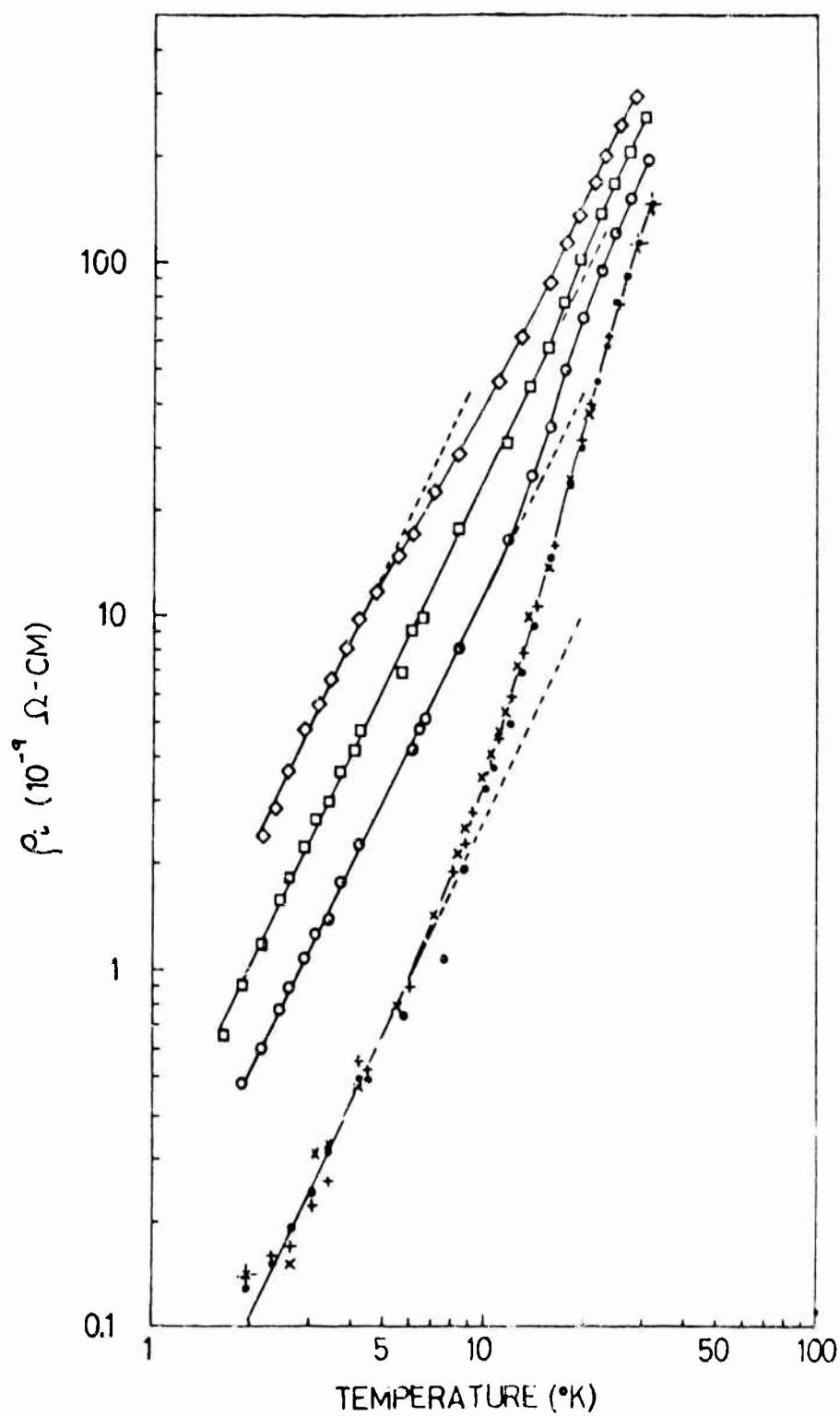
Fig. 9 - The ideal electrical resistivity as a function of temperature \bullet+x , three high purity samples of pure palladium; \circ , Pd-1/2%Ni; \square , Pd-1%Ni; \diamond , Pd-1.66%Ni.
